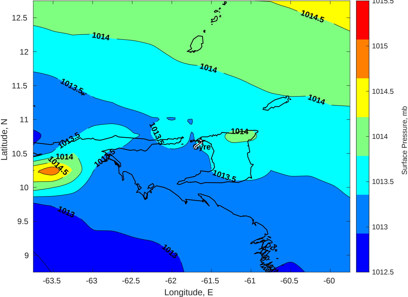
Surface Pressure (mb) for Gyre at 09-Jan-2026 00:00:00
