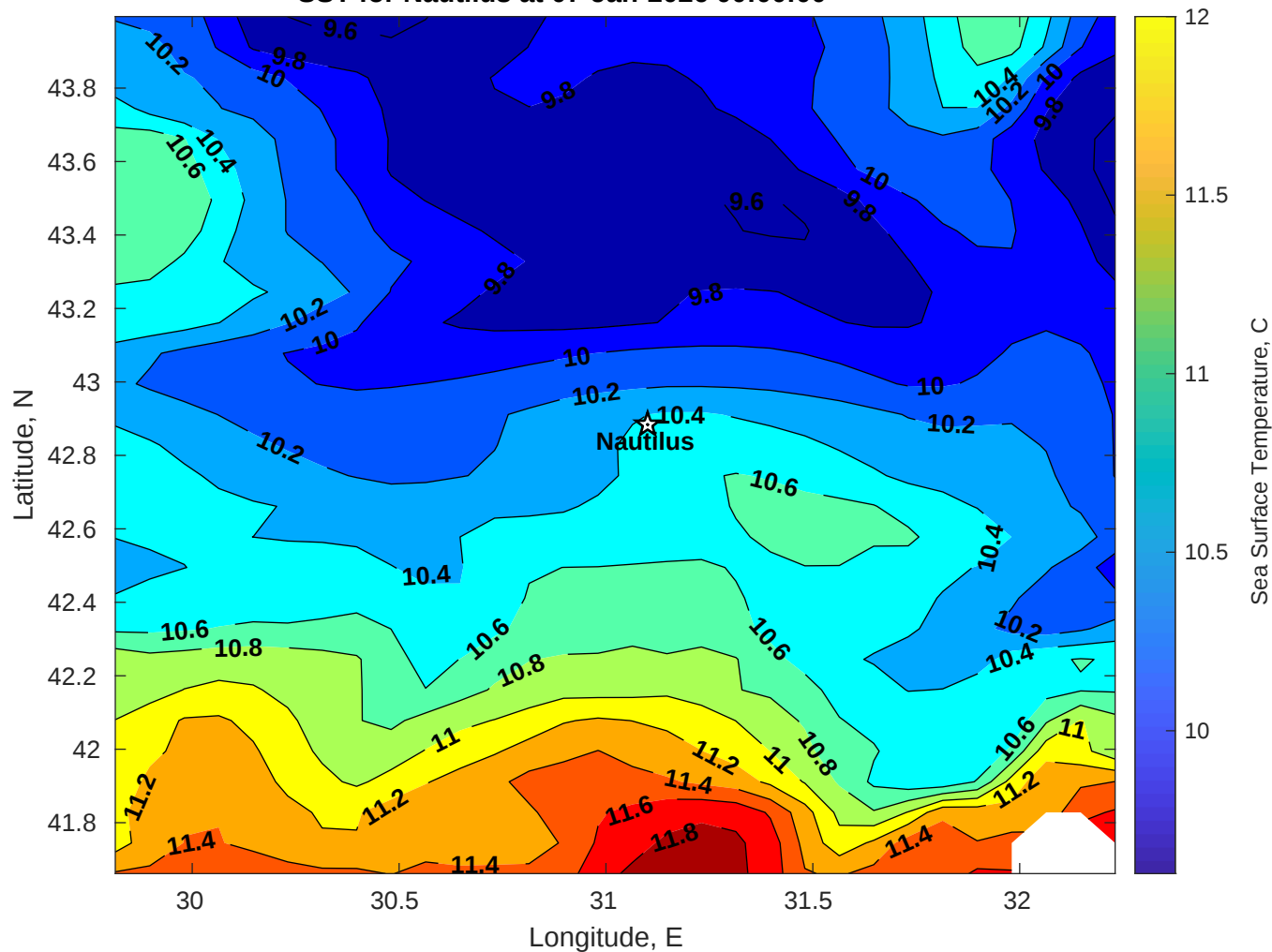
SST for Nautilus at 07-Jan-2026 00:00:00
