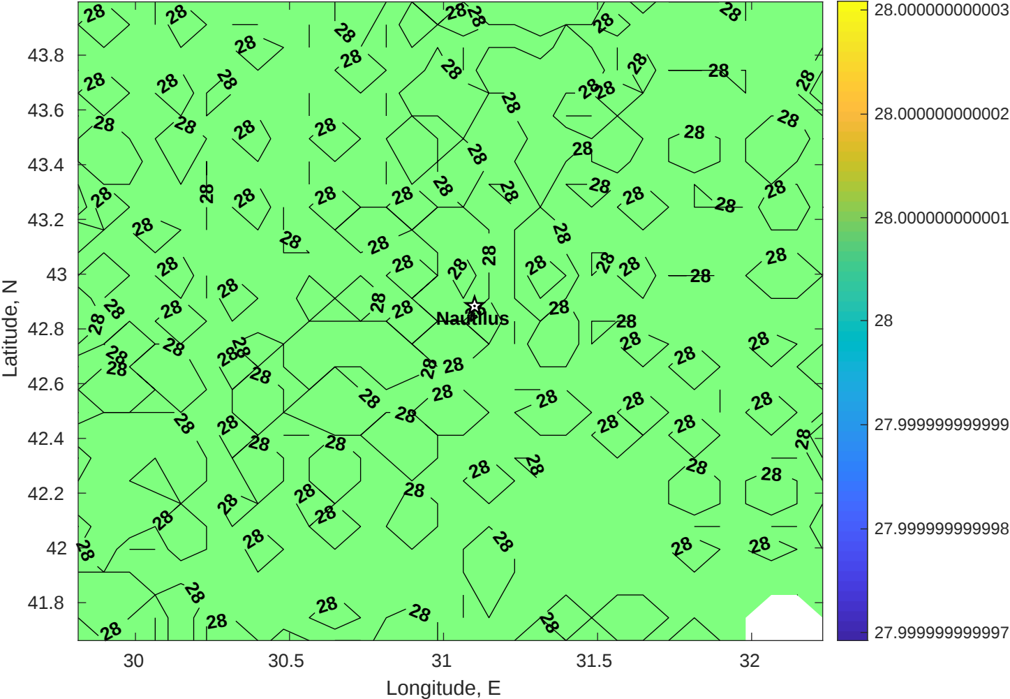
Surface Salinity for Nautilus at 07-Jan-2026 00:00:00
