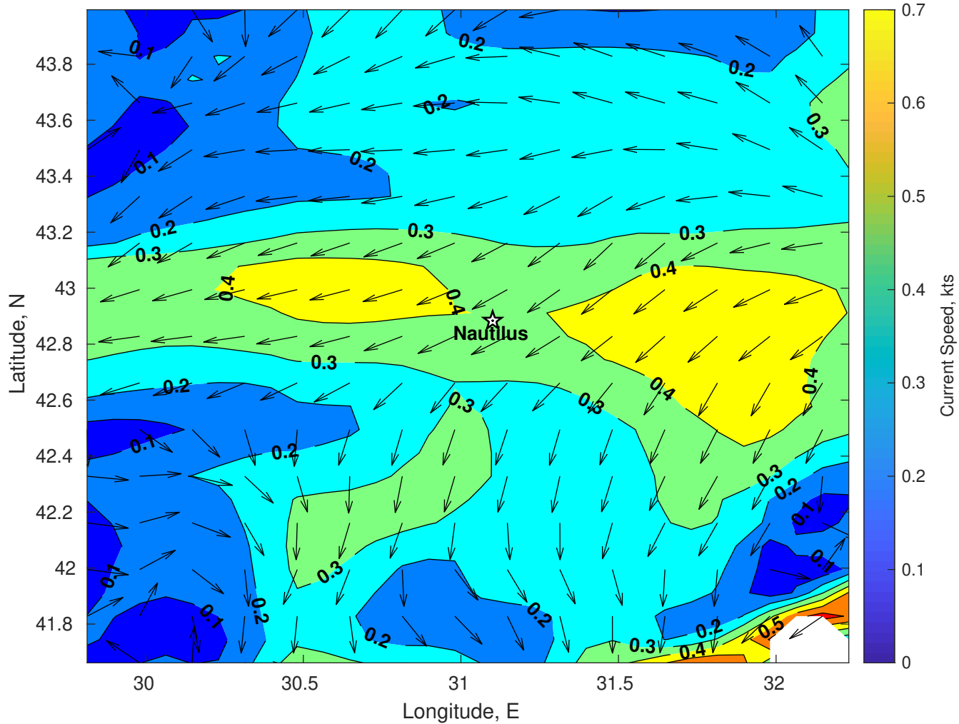
Surface Currents for Nautilus at 07-Jan-2026 00:00:00
