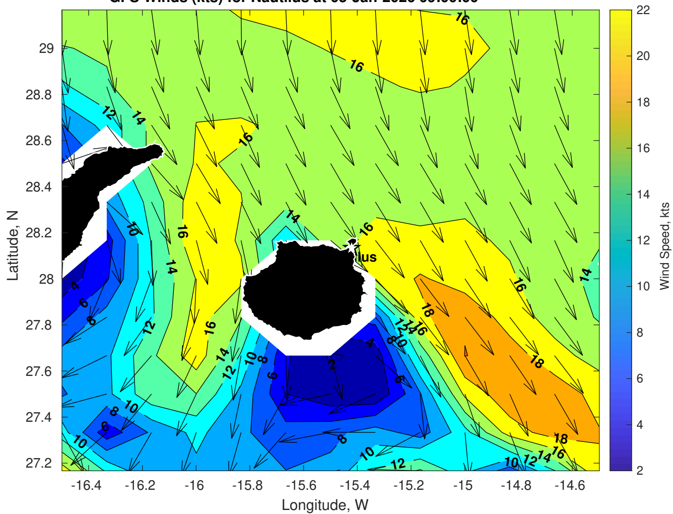
GFS Winds (kts) for Nautilus at 05-Jan-2026 09:00:00
