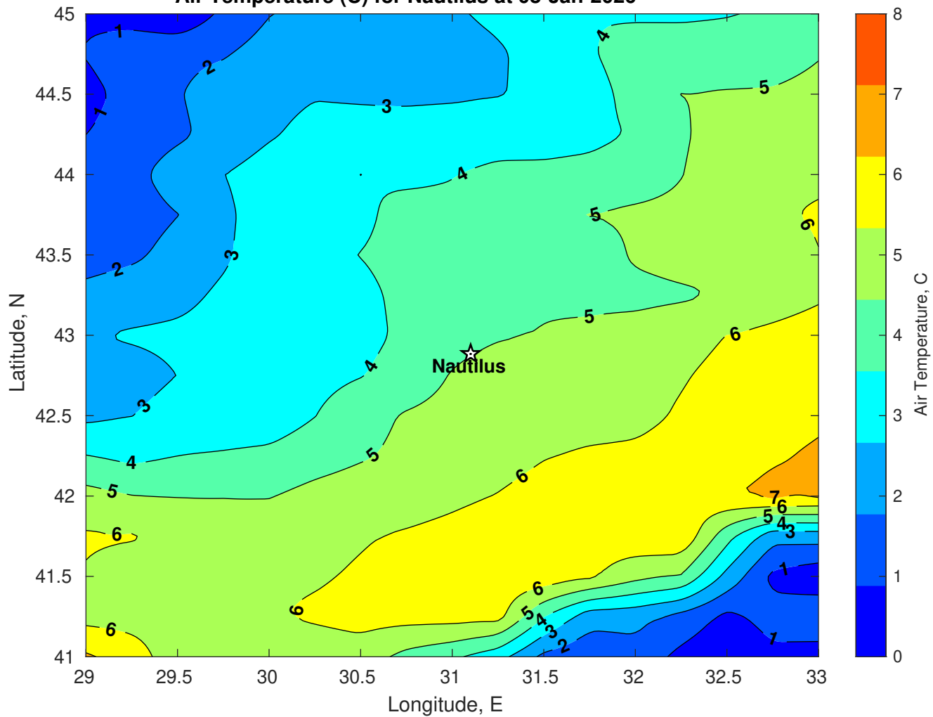
Air Temperature (C) for Nautilus at 08-Jan-2026
