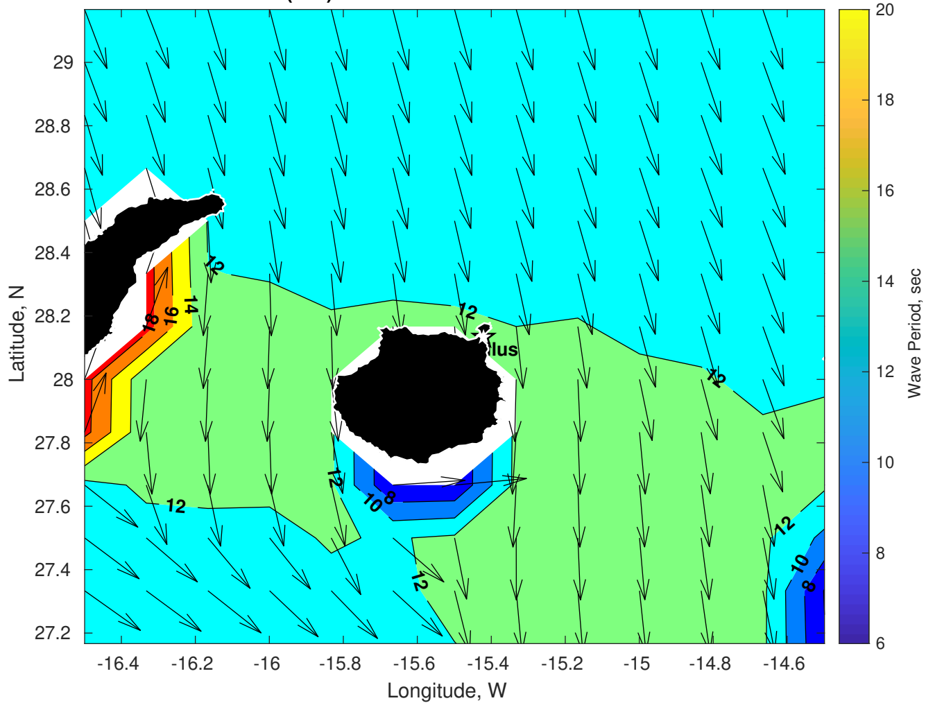
GFS Wave Period (sec) for Nautilus at 05-Jan-2026 09:00:00
