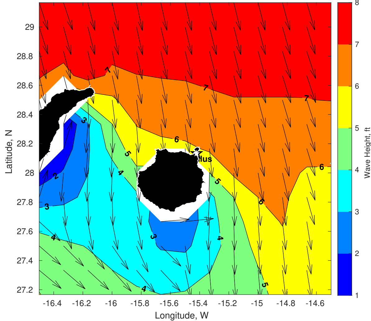
GFS Wave Height (ft) for Nautilus at 05-Jan-2026 09:00:00
