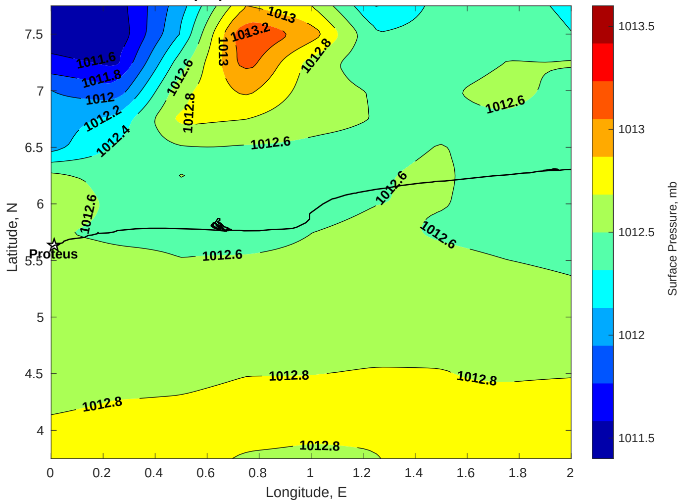
Surface Pressure (mb) for Proteus at 08-Jan-2026 00:00:00
