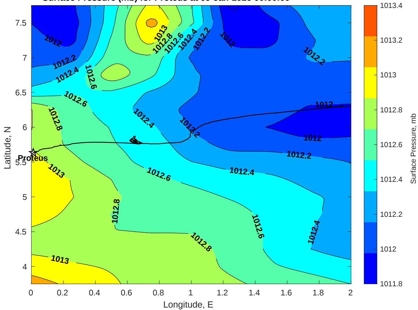
Surface Pressure (mb) for Proteus at 09-Jan-2026 00:00:00
