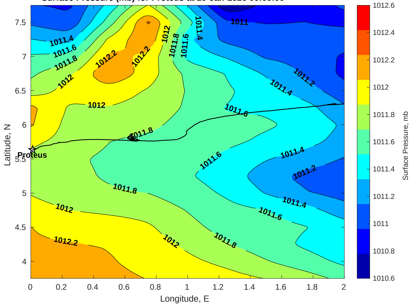
Surface Pressure (mb) for Proteus at 10-Jan-2026 00:00:00
