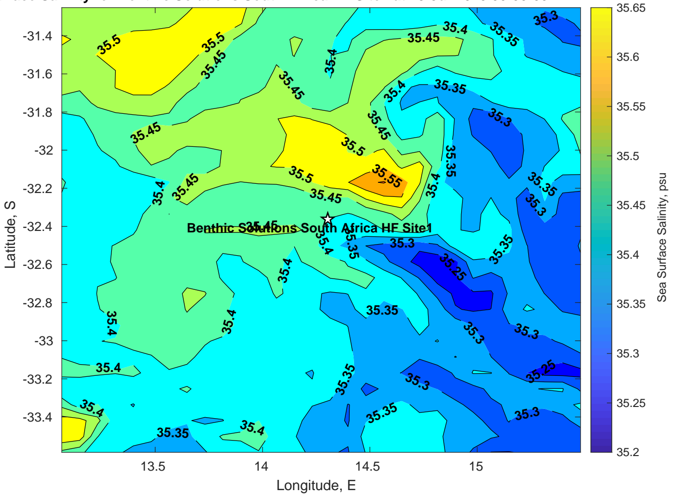
Surface Salinity for Benthic Solutions South Africa HF Site1 at 13-Jul-2025 00:00:00
