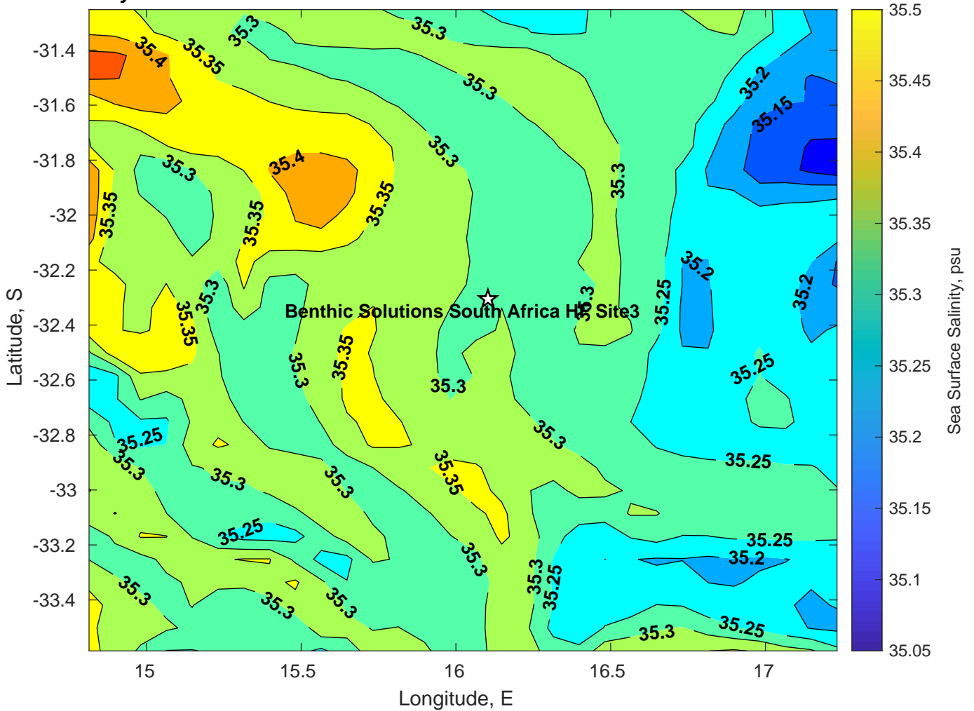
Surface Salinity for Benthic Solutions South Africa HF Site3 at 13-Jul-2025 00:00:00
