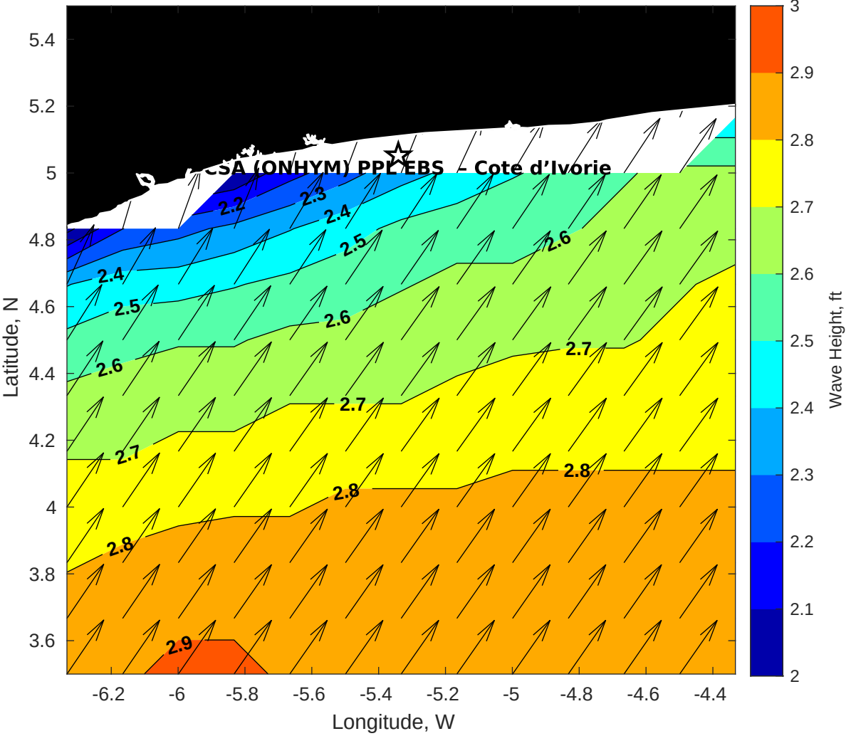
GFS Wave Height (ft) for CSA (ONHYM) PPL EBS - Cote d'Ivoire at 09-Jan-2026 09:00:00
