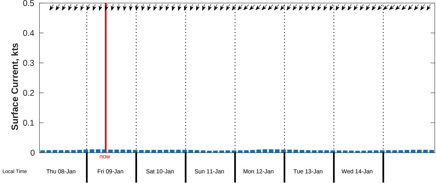
Surface Current Forecast for CSA (ONHYM) PPL EBS - Ghana from 08-Jan-2026 00:00:00 to 16-Jan-2026 00:00:00
