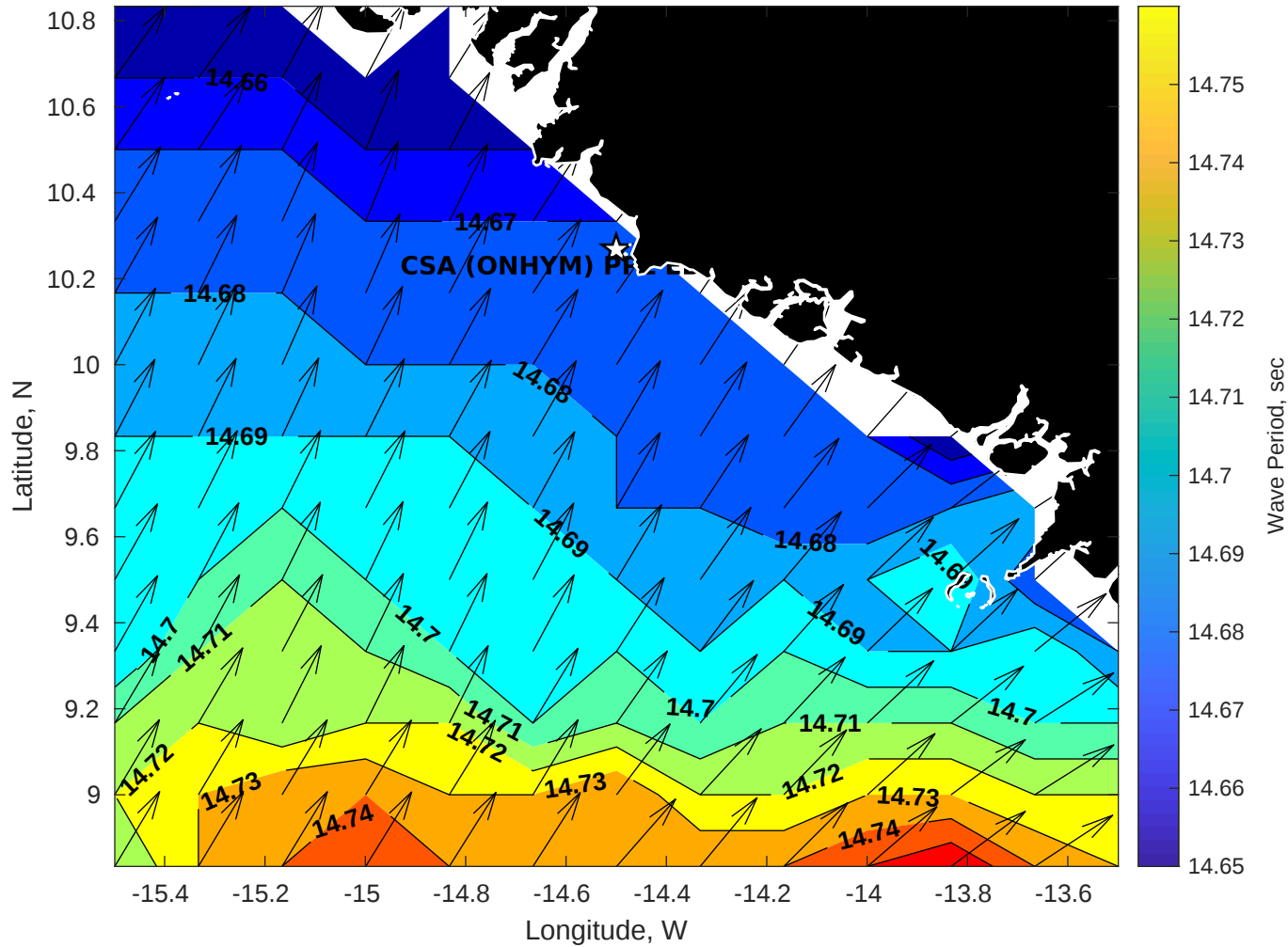
GFS Wave Period (sec) for CSA (ONHYM) PPL EBS - Guinea at 09-Jan-2026 09:00:00
