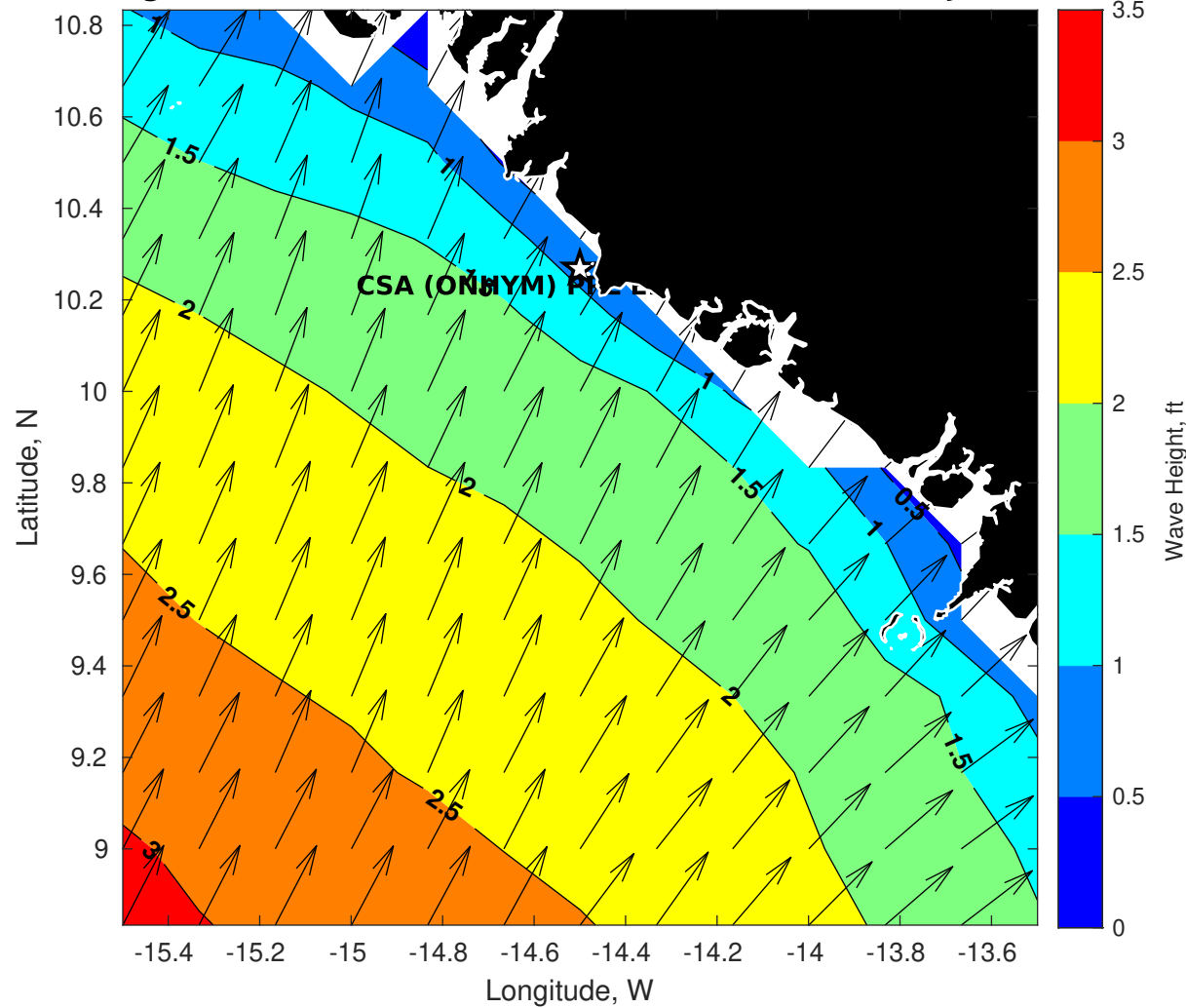
GFS Wave Height (ft) for CSA (ONHYM) PPL EBS - Guinea at 09-Jan-2026 09:00:00
