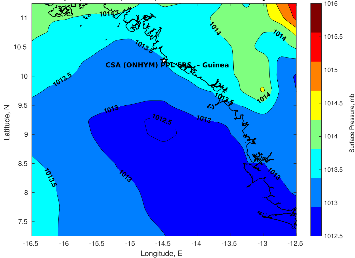
Surface Pressure (mb) for CSA (ONHYM) PPL EBS - Guinea at 09-Jan-2026 00:00:00
