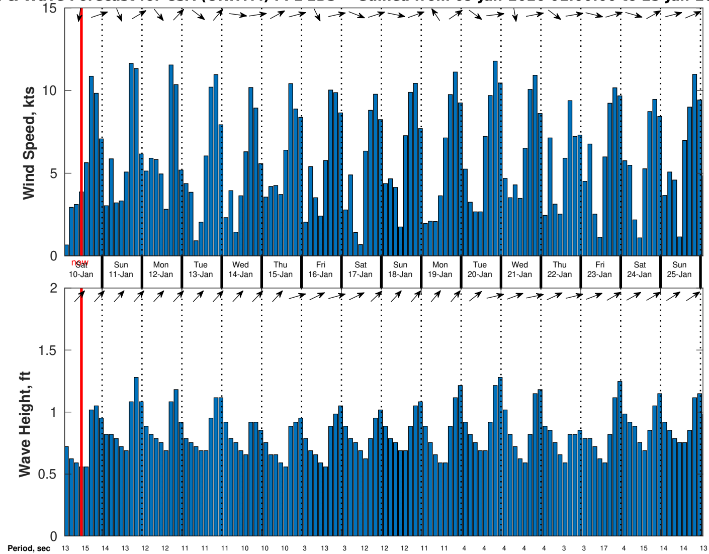
Wind & Wave Forecast for CSA (ONHYM) PPL EBS - Guinea from 09-Jan-2026 01:00:00 to 25-Jan-2026 01:00:00
