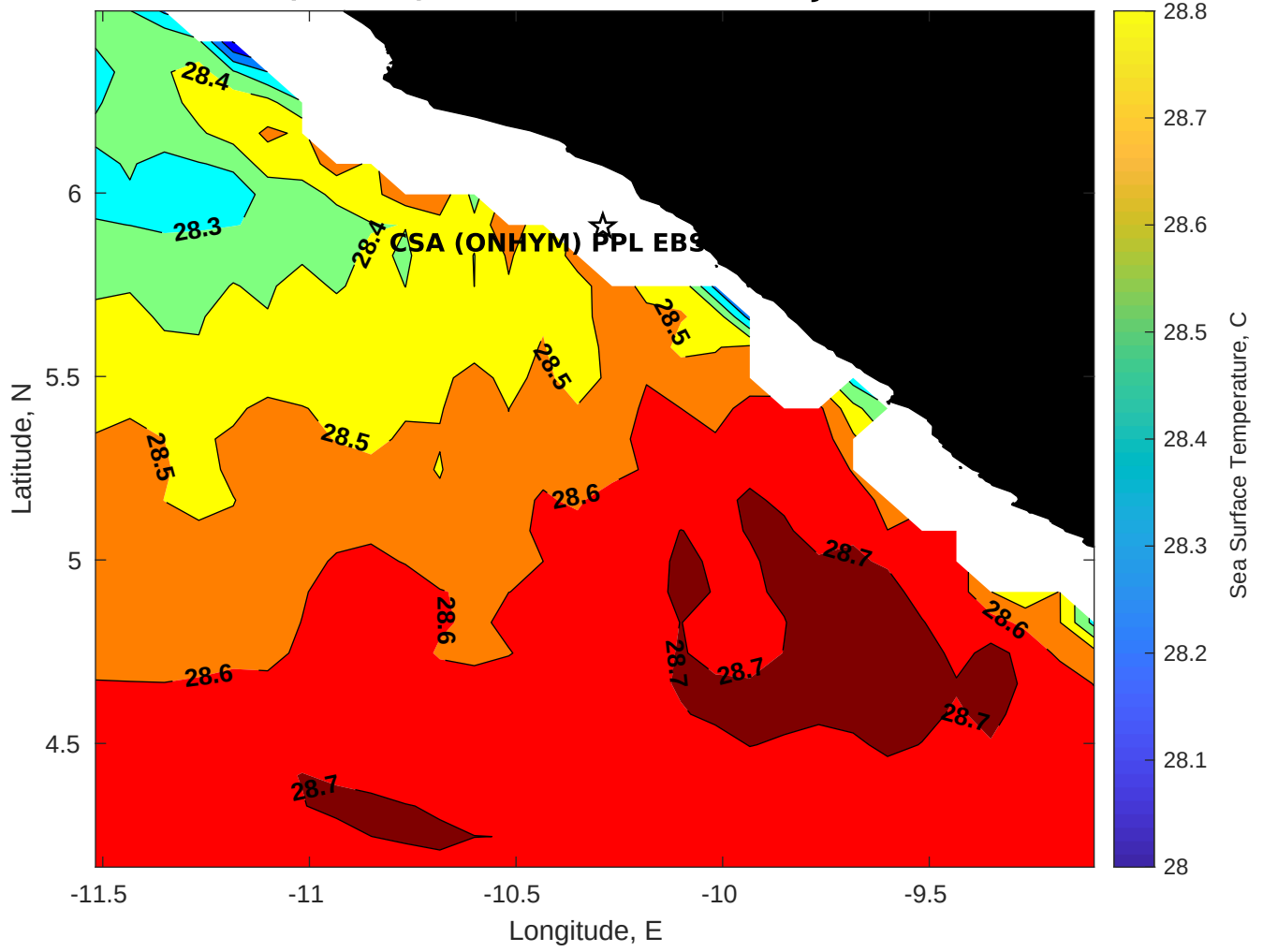
SST for CSA (ONHYM) PPL EBS - Liberia at 08-Jan-2026 00:00:00
