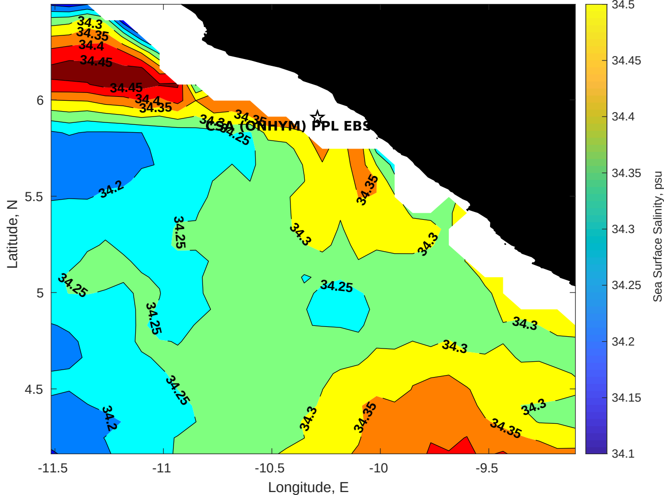
Surface Salinity for CSA (ONHYM) PPL EBS - Liberia at 08-Jan-2026 00:00:00
