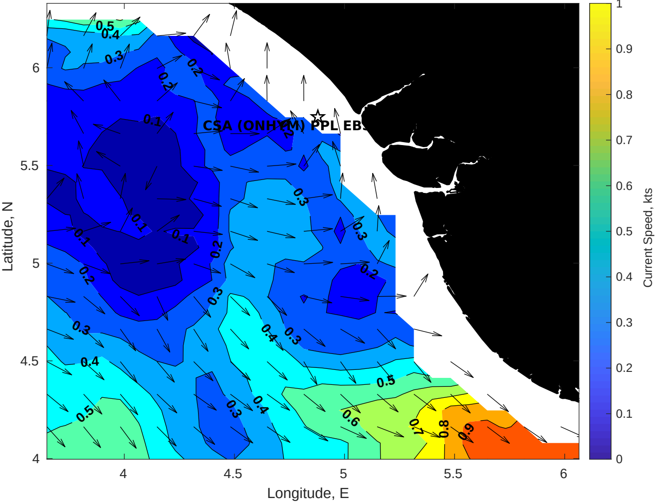
Surface Currents for CSA (ONHYM) PPL EBS - Nigeria at 08-Jan-2026 00:00:00
