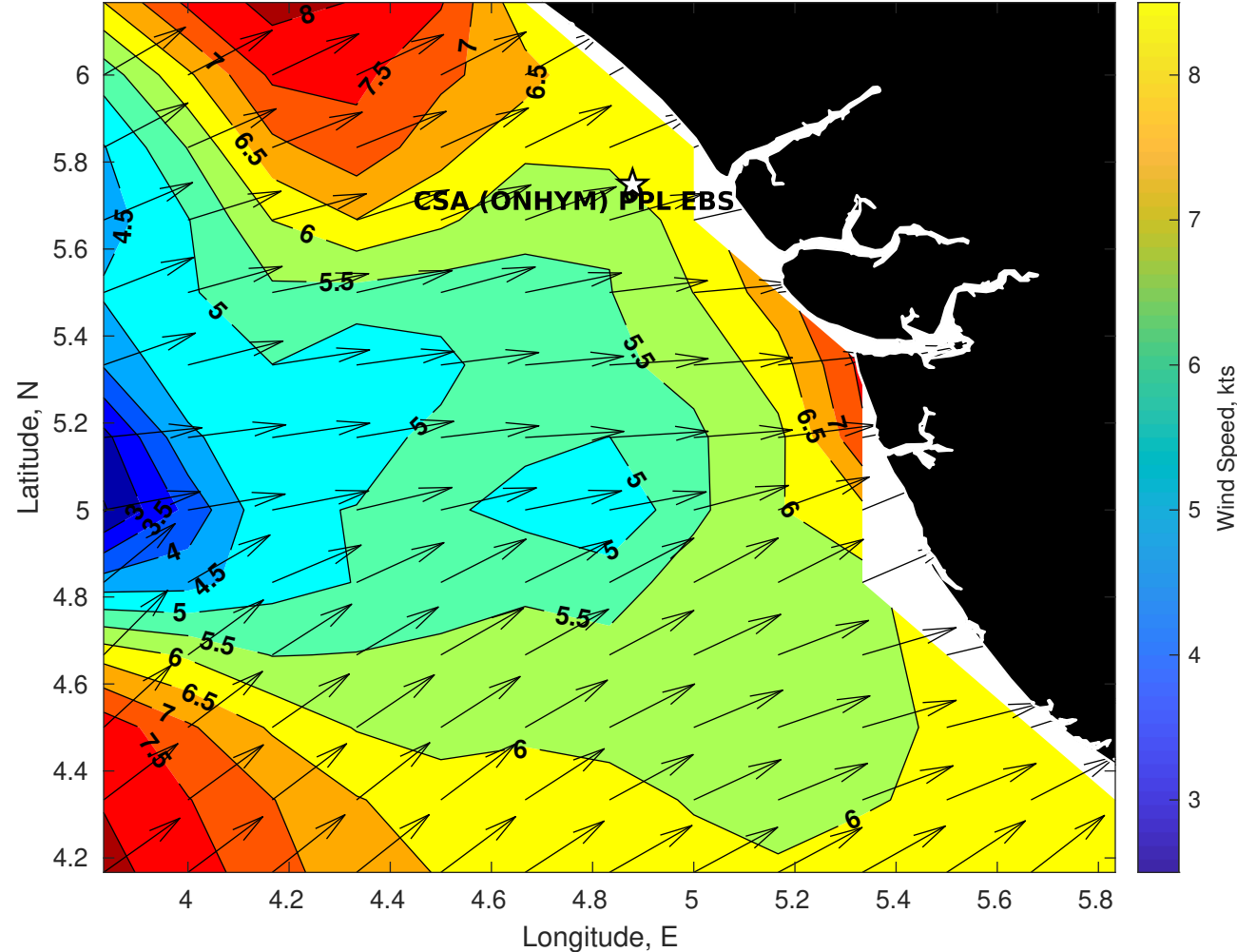
GFS Winds (kts) for CSA (ONHYM) PPL EBS - Nigeria at 09-Jan-2026 09:00:00
