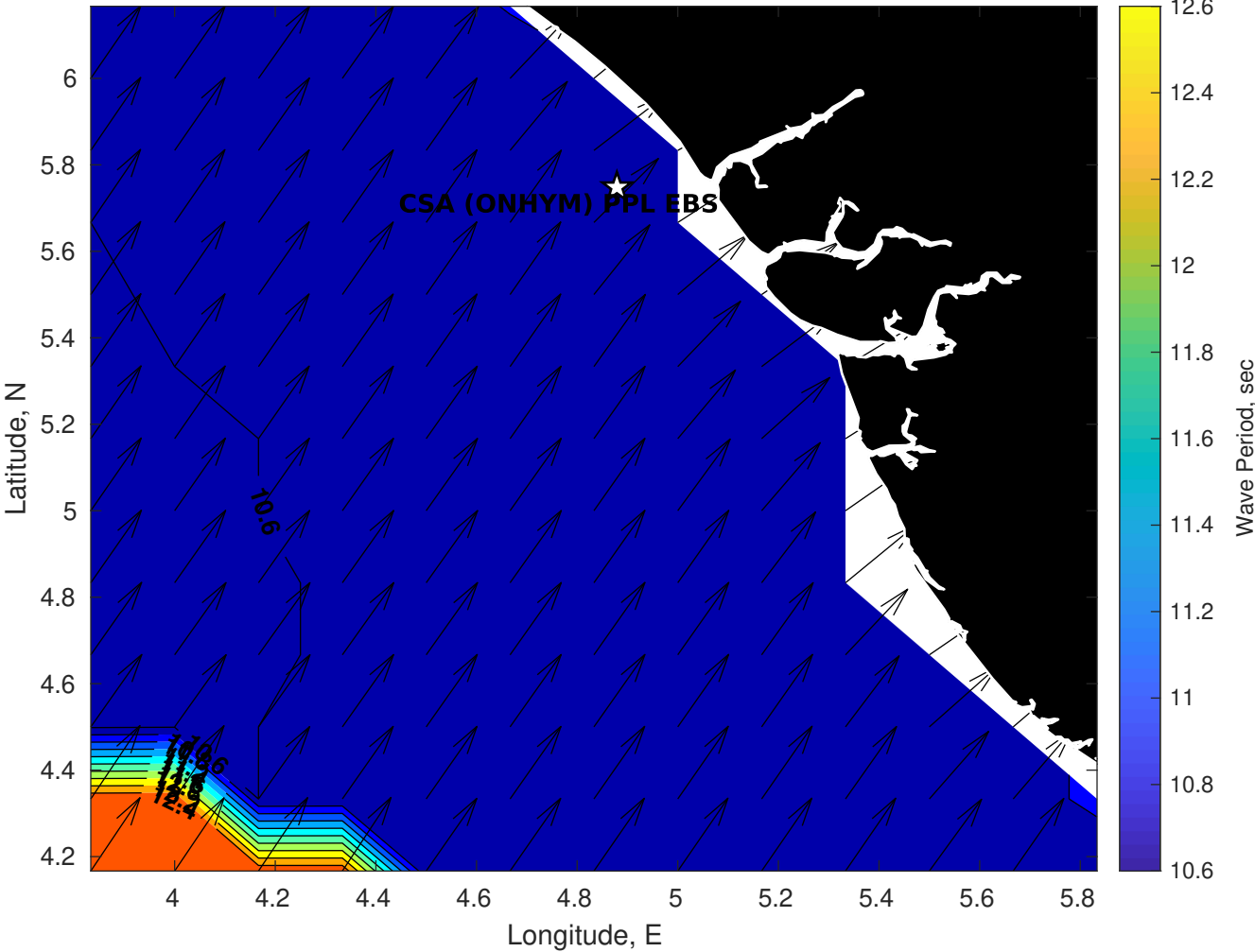
GFS Wave Period (sec) for CSA (ONHYM) PPL EBS - Nigeria at 09-Jan-2026 09:00:00
