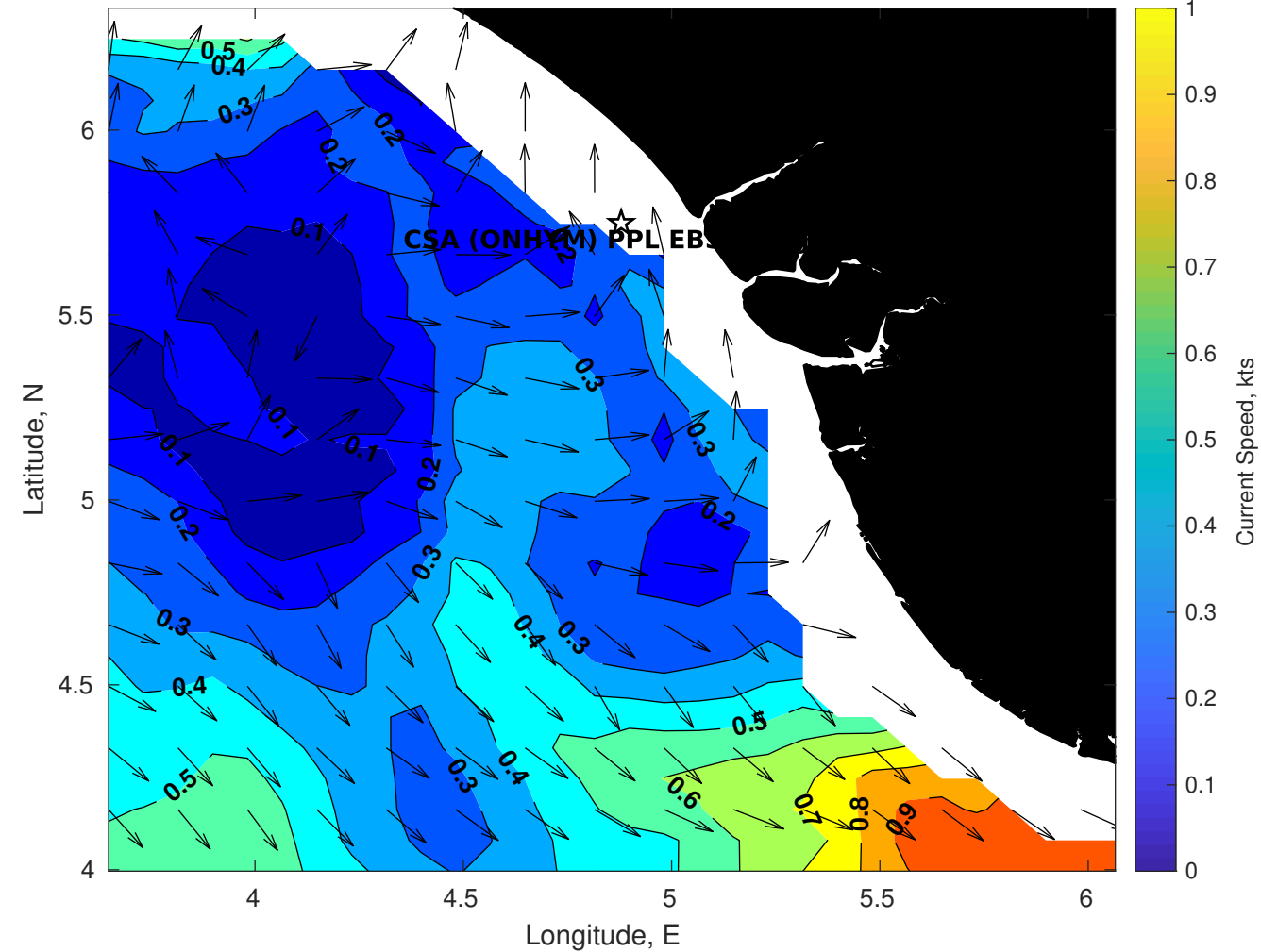
Surface Currents for CSA (ONHYM) PPL EBS - Nigeria at 08-Jan-2026 00:00:00
