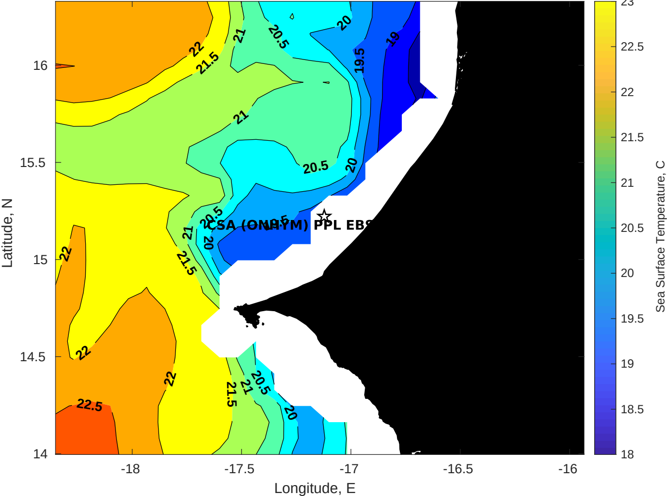
SST for CSA (ONHYM) PPL EBS - Senegal at 08-Jan-2026 00:00:00
