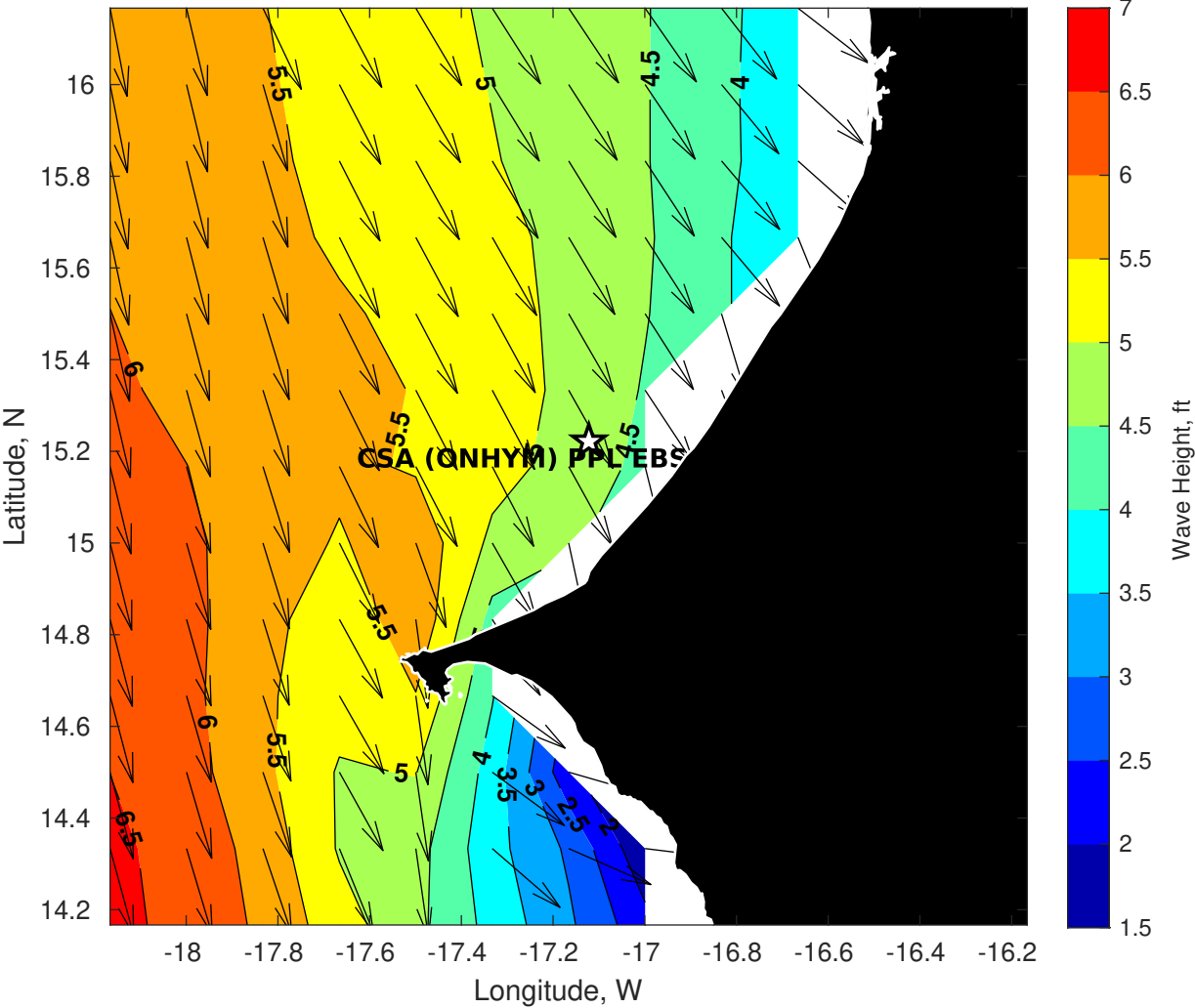
GFS Wave Height (ft) for CSA (ONHYM) PPL EBS - Senegal at 09-Jan-2026 09:00:00
