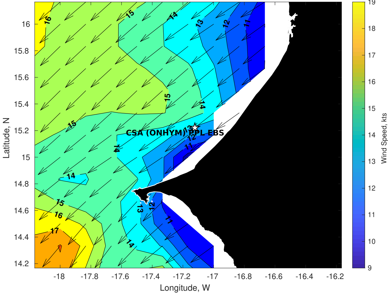
GFS Winds (kts) for CSA (ONHYM) PPL EBS - Senegal at 09-Jan-2026 09:00:00
