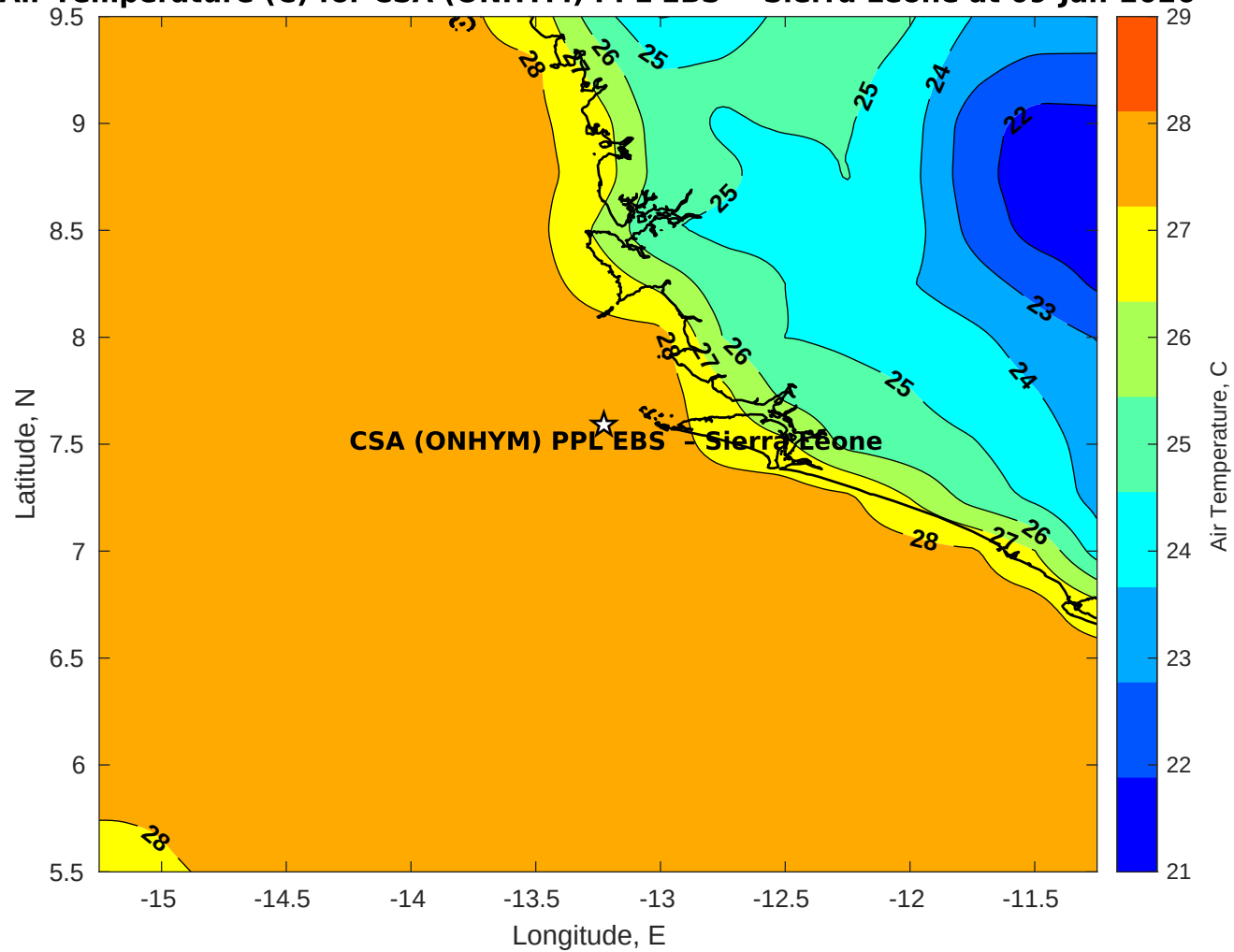
Air Temperature (C) for CSA (ONHYM) PPL EBS - Sierra Leone at 09-Jan-2026
