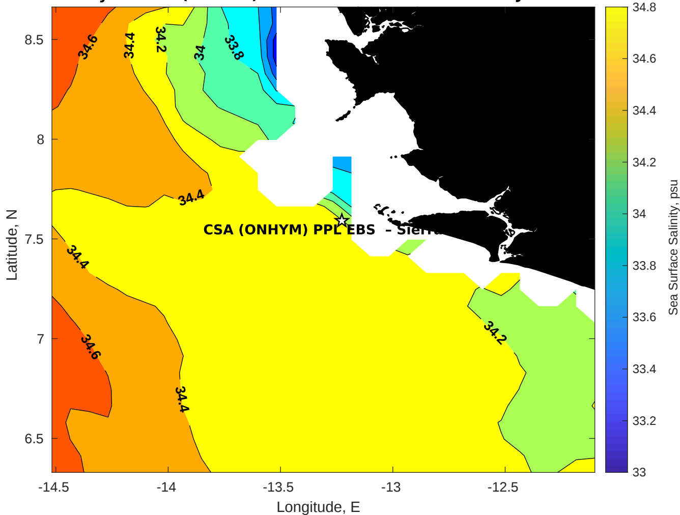
Surface Salinity for CSA (ONHYM) PPL EBS - Sierra Leone at 08-Jan-2026 00:00:00
