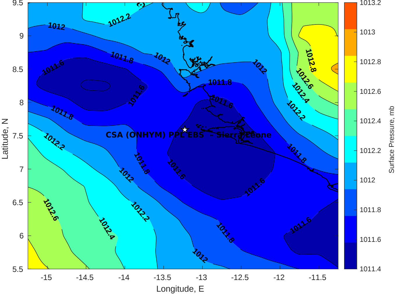
Surface Pressure (mb) for CSA (ONHYM) PPL EBS - Sierra Leone at 11-Jan-2026 00:00:00
