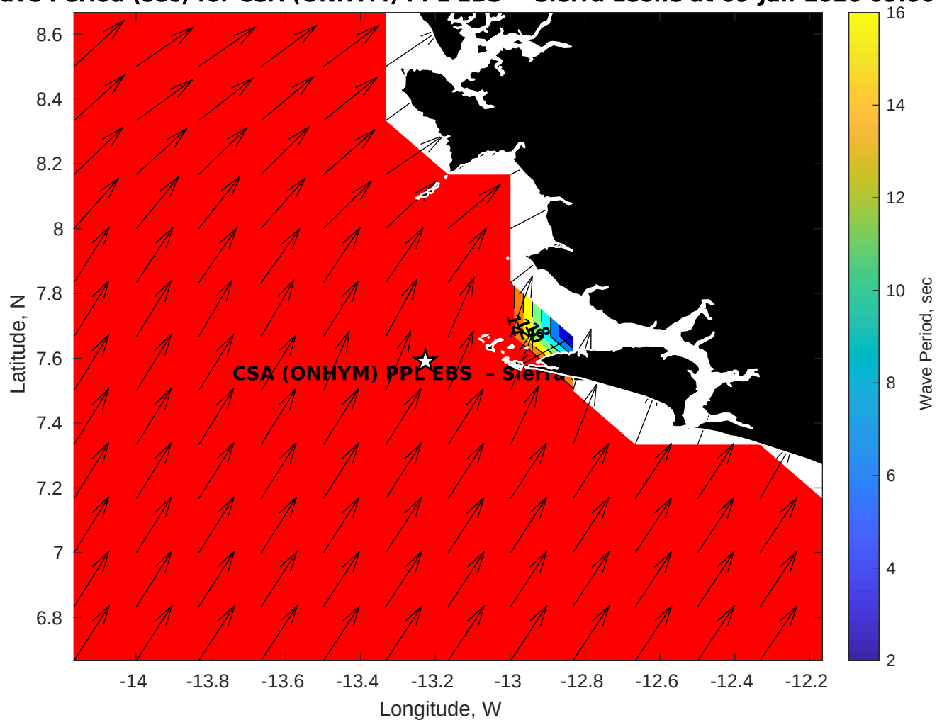
GFS Wave Period (sec) for CSA (ONHYM) PPL EBS - Sierra Leone at 09-Jan-2026 09:00:00
