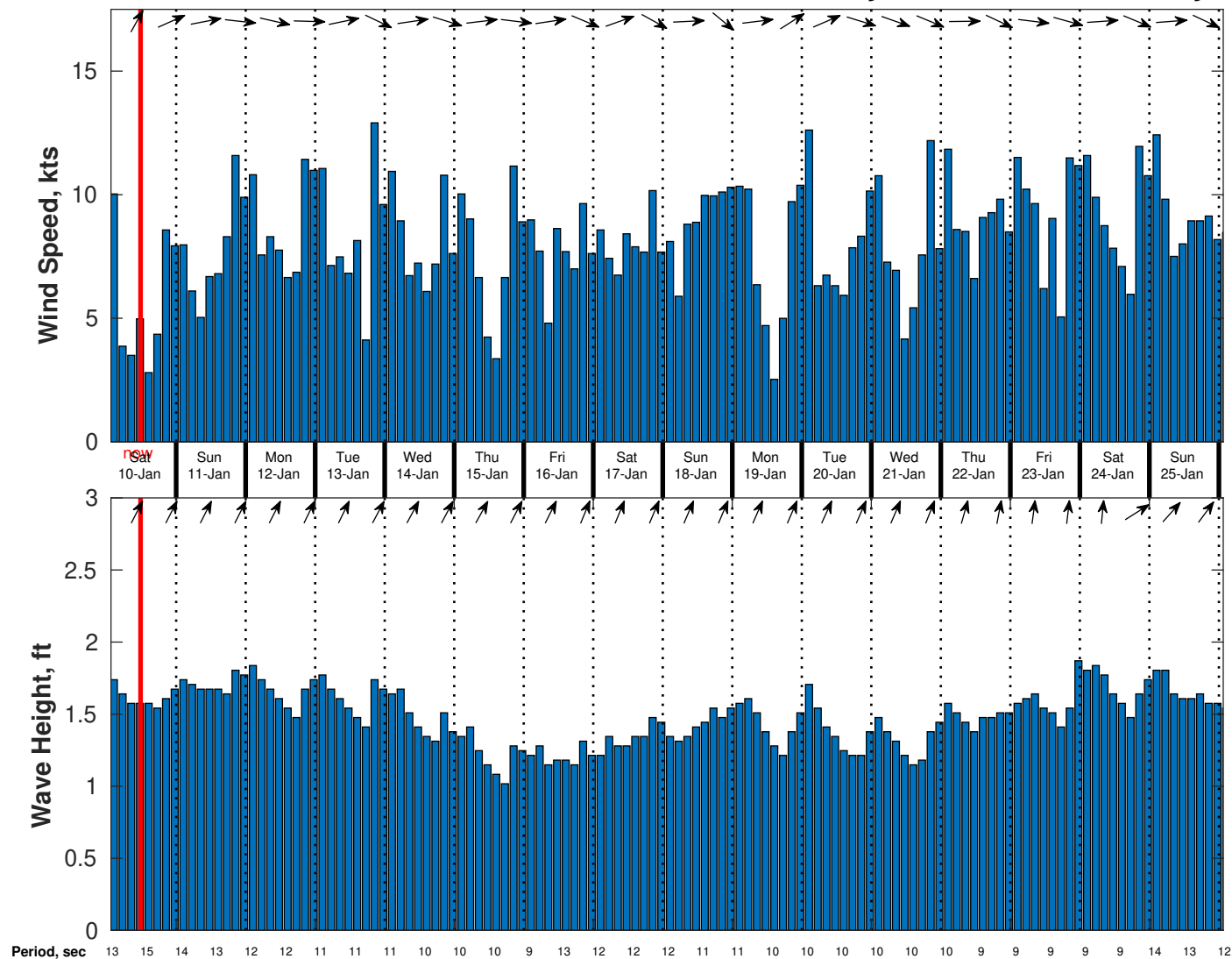
Wind & Wave Forecast for CSA (ONHYM) PPL EBS - Sierra Leone from 09-Jan-2026 01:00:00 to 25-Jan-2026 01:00:00
