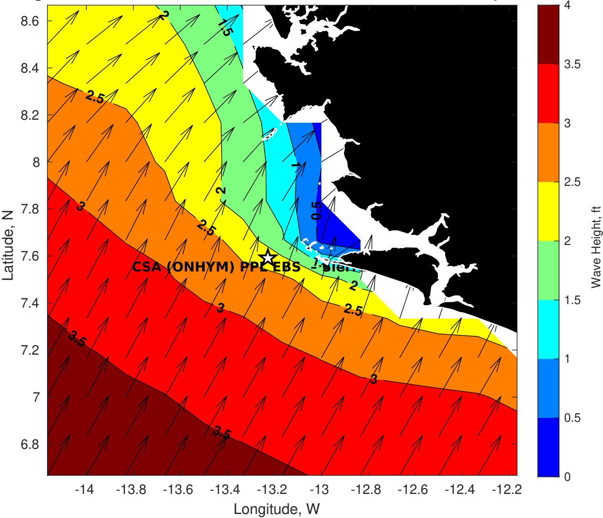
GFS Wave Height (ft) for CSA (ONHYM) PPL EBS - Sierra Leone at 09-Jan-2026 09:00:00
