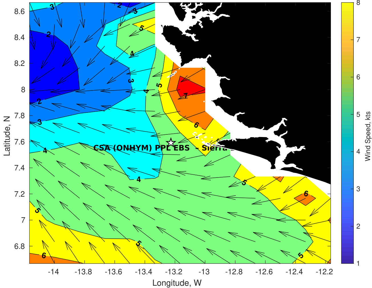
GFS Winds (kts) for CSA (ONHYM) PPL EBS - Sierra Leone at 09-Jan-2026 09:00:00
