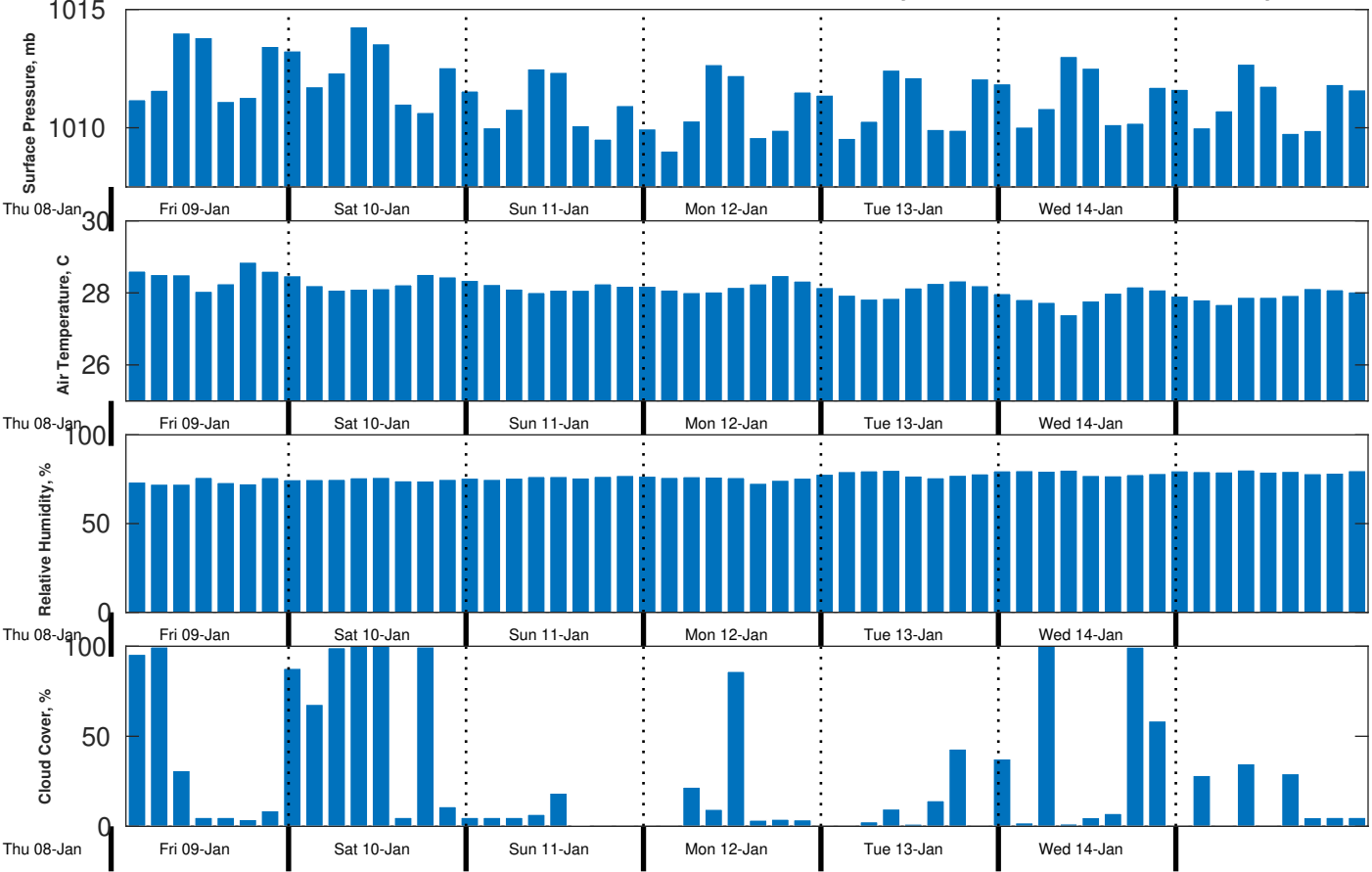
Met Forecast for CSA (ONHYM) PPL EBS - Sierra Leone from 09-Jan-2026 00:00:00 to 16-Jan-2026 00:00:00
