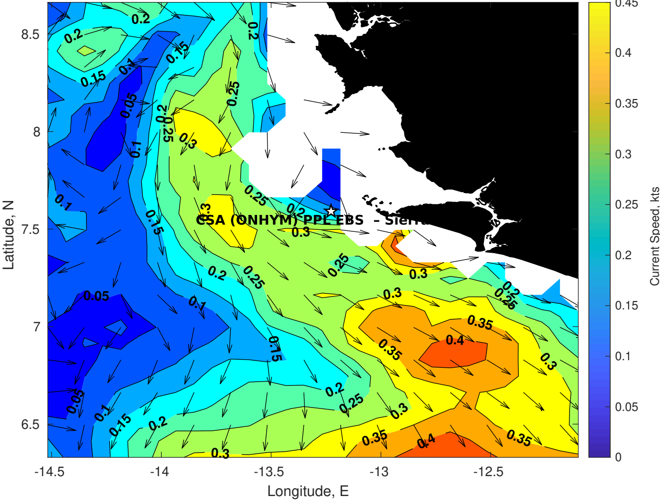
Surface Currents for CSA (ONHYM) PPL EBS - Sierra Leone at 08-Jan-2026 00:00:00
