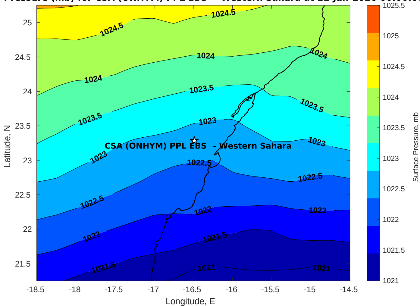
Surface Pressure (mb) for CSA (ONHYM) PPL EBS - Western Sahara at 11-Jan-2026 00:00:00
