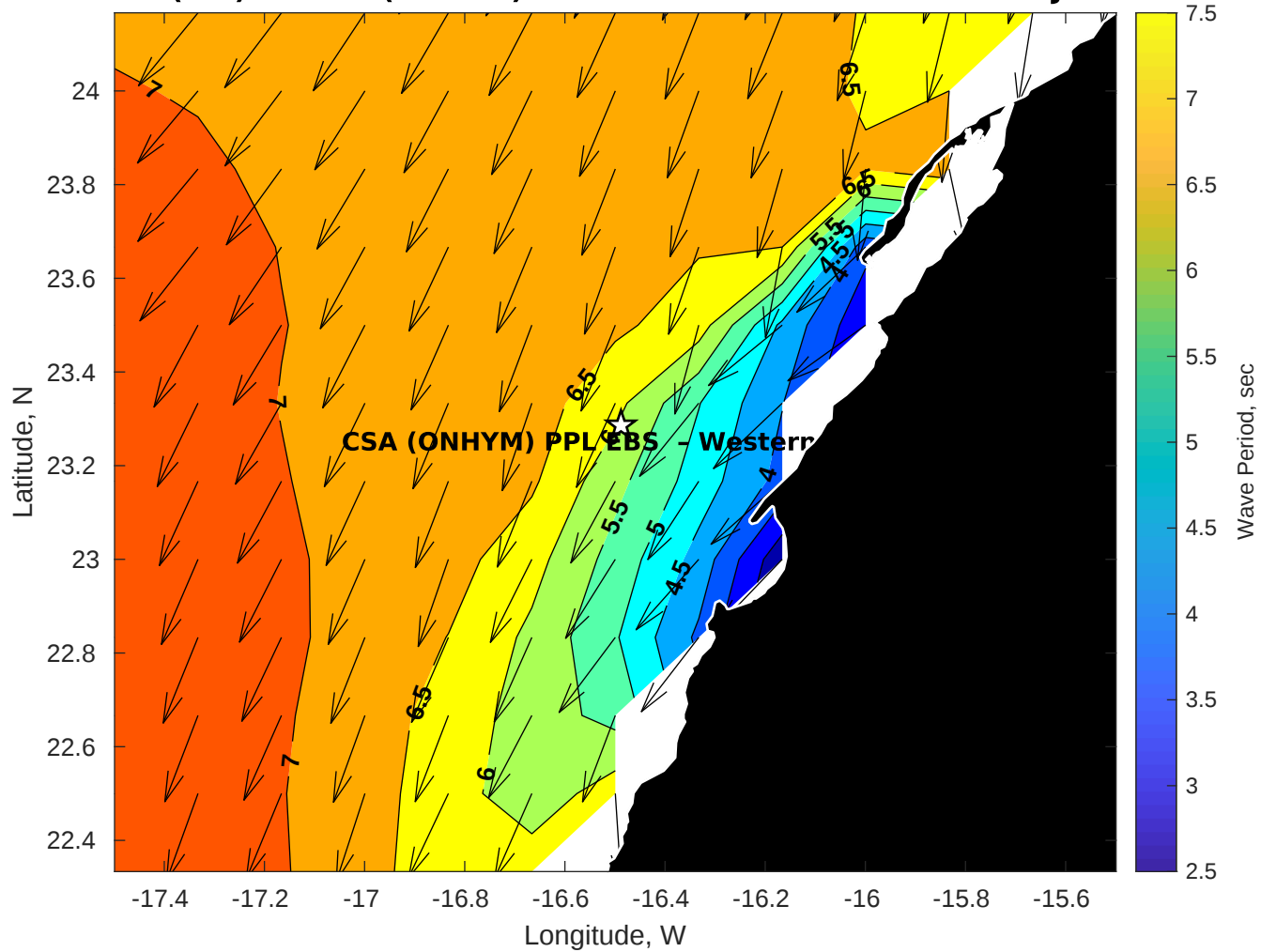
GFS Wave Period (sec) for CSA (ONHYM) PPL EBS - Western Sahara at 09-Jan-2026 09:00:00
