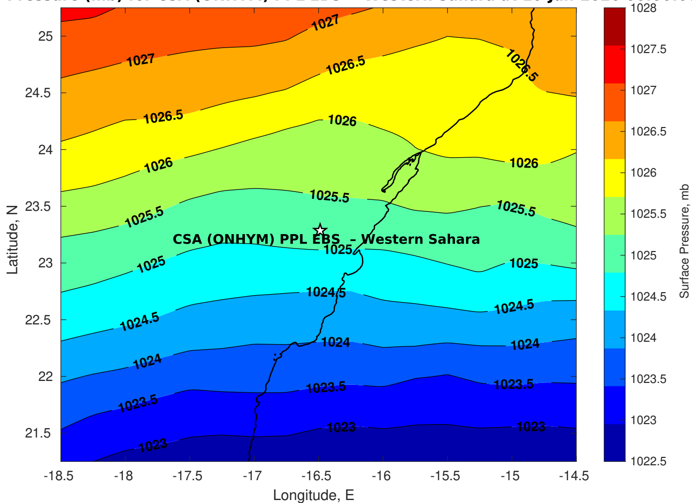
Surface Pressure (mb) for CSA (ONHYM) PPL EBS - Western Sahara at 10-Jan-2026 00:00:00
