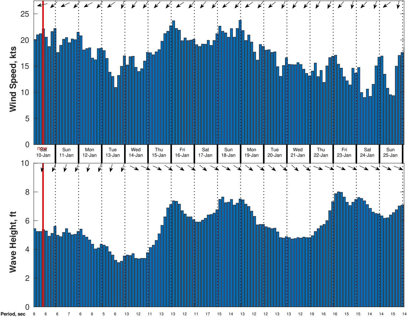
Wind & Wave Forecast for CSA (ONHYM) PPL EBS - Western Sahara from 09-Jan-2026 01:00:00 to 25-Jan-2026 01:00:00
