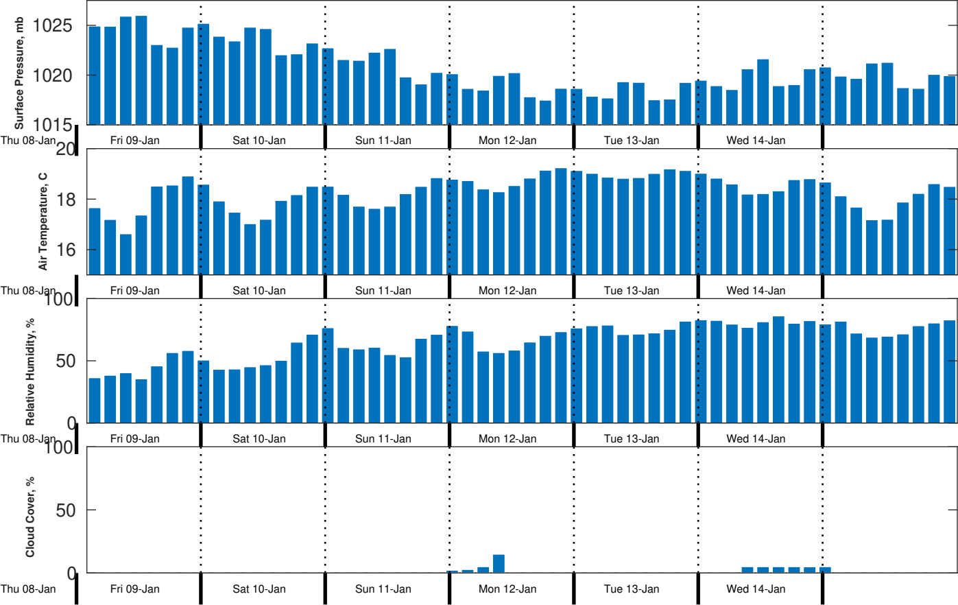
Met Forecast for CSA (ONHYM) PPL EBS - Western Sahara from 09-Jan-2026 00:00:00 to 16-Jan-2026 00:00:00
