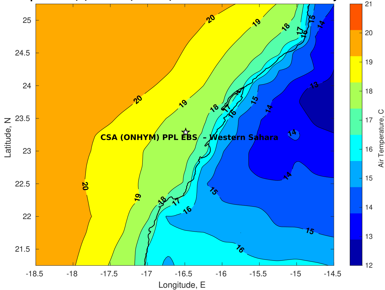
Air Temperature (C) for CSA (ONHYM) PPL EBS - Western Sahara at 09-Jan-2026
