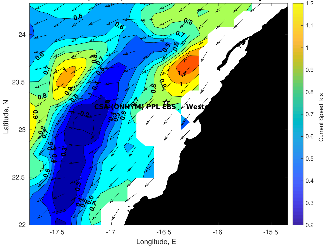
Surface Currents for CSA (ONHYM) PPL EBS - Western Sahara at 08-Jan-2026 00:00:00
