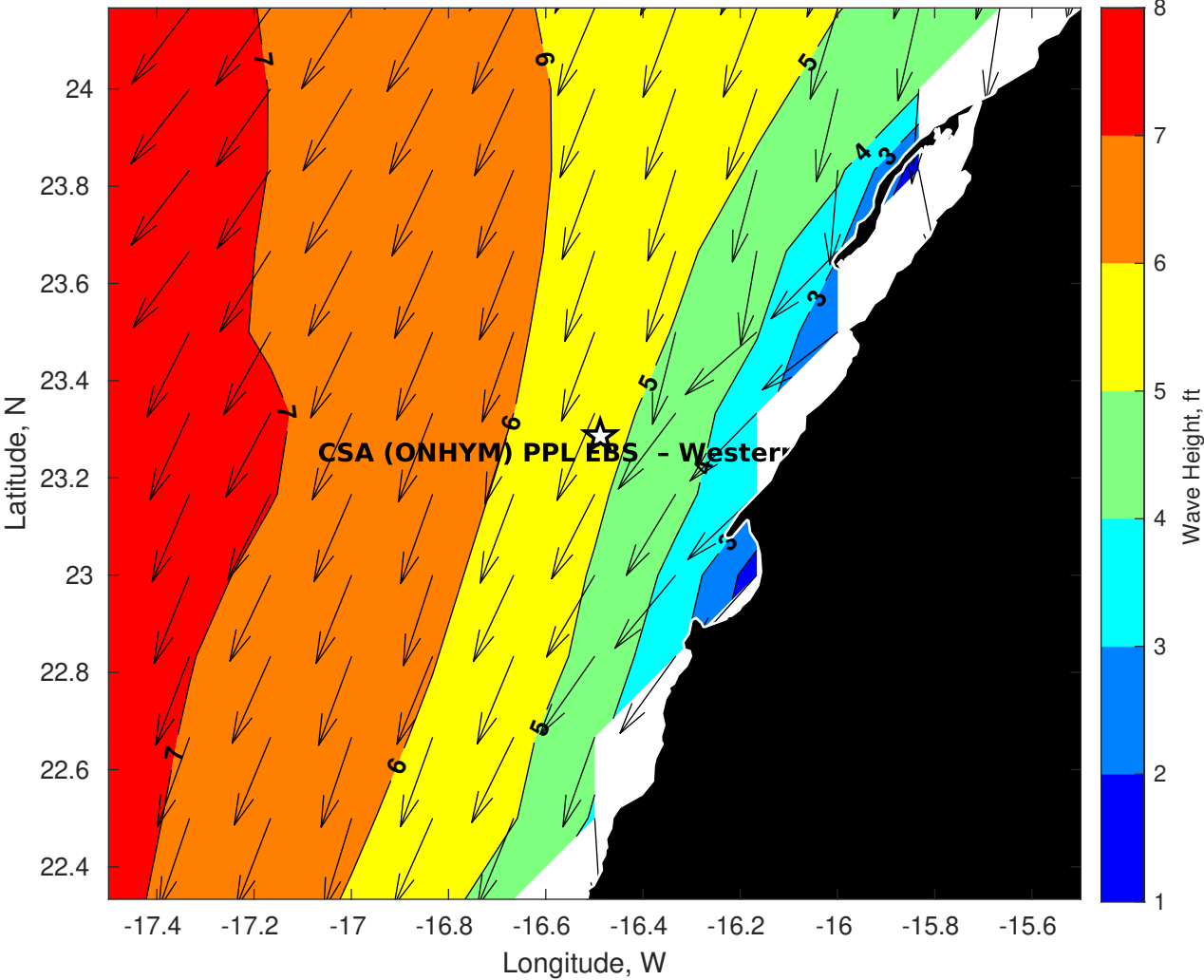
GFS Wave Height (ft) for CSA (ONHYM) PPL EBS - Western Sahara at 09-Jan-2026 09:00:00
