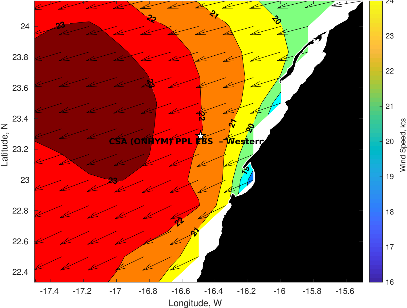
GFS Winds (kts) for CSA (ONHYM) PPL EBS - Western Sahara at 09-Jan-2026 09:00:00
