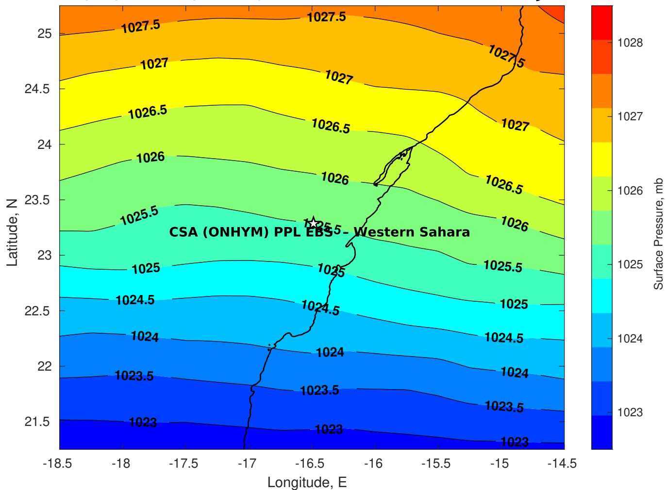
Surface Pressure (mb) for CSA (ONHYM) PPL EBS - Western Sahara at 09-Jan-2026 00:00:00
