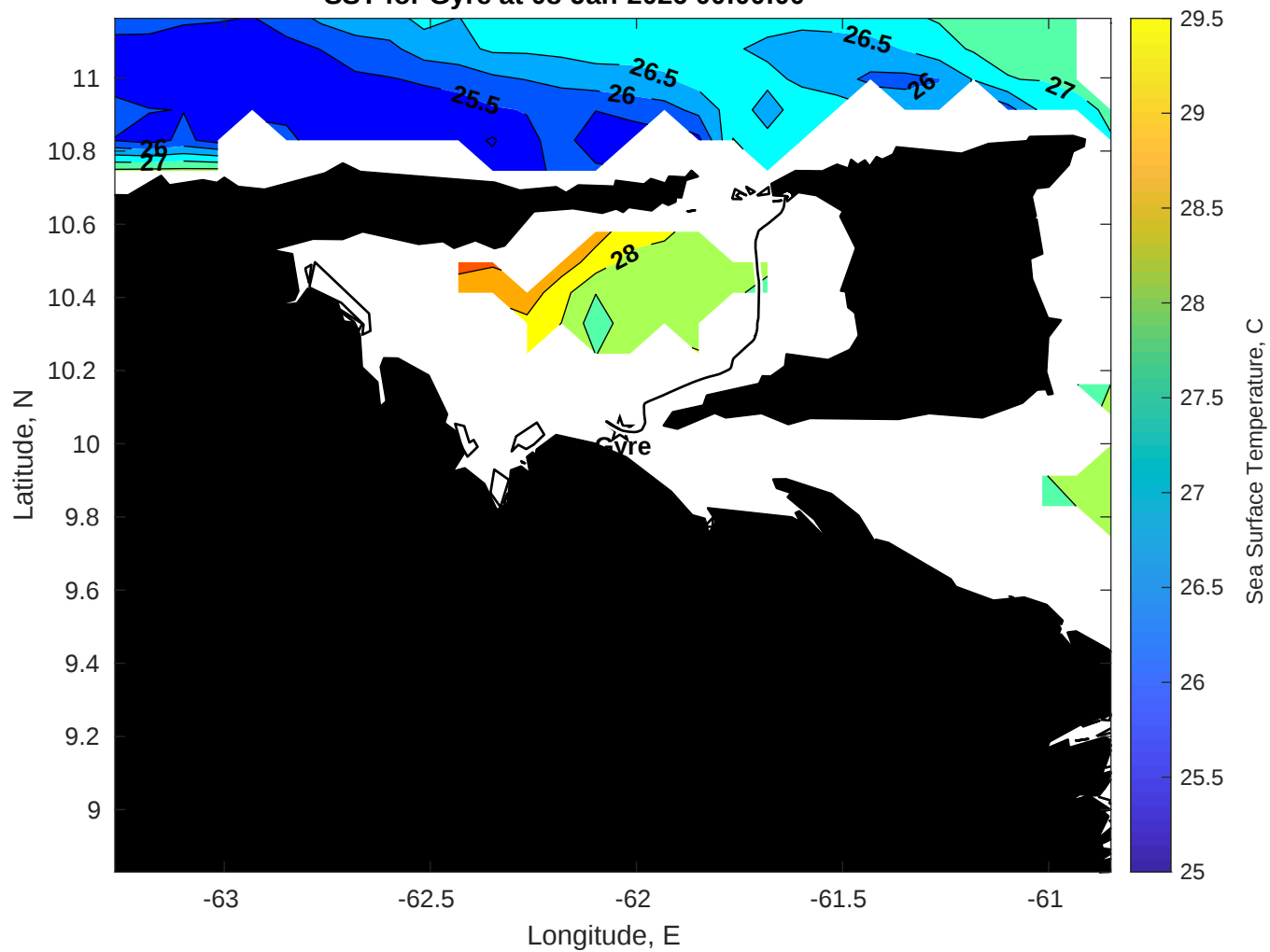
SST for Gyre at 08-Jan-2026 00:00:00
