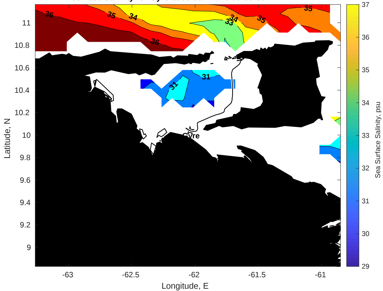
Surface Salinity for Gyre at 08-Jan-2026 00:00:00
