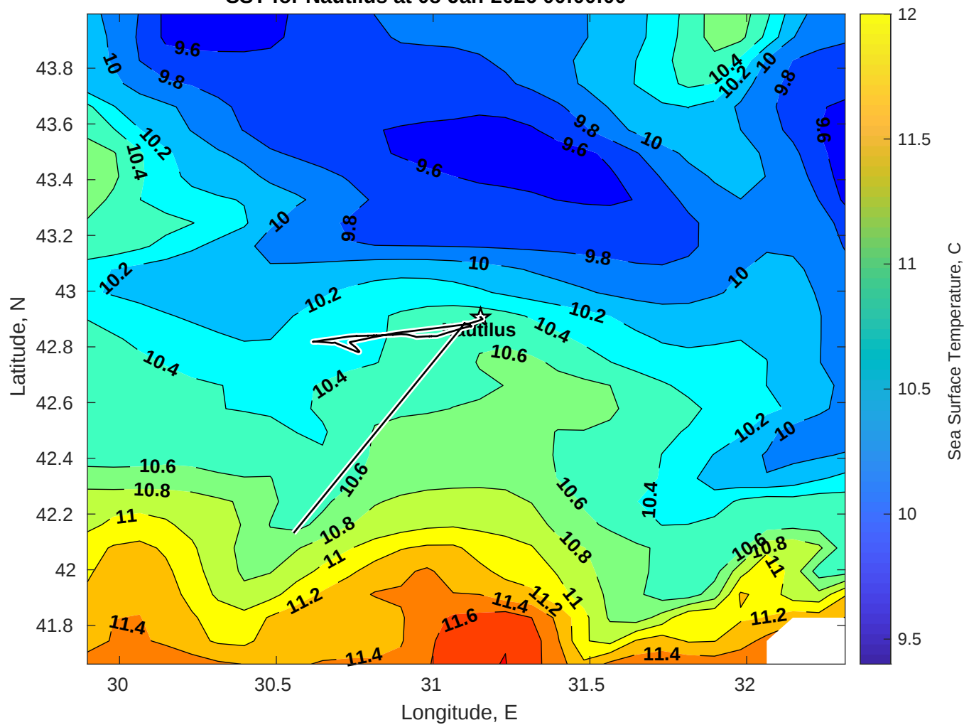
SST for Nautilus at 08-Jan-2026 00:00:00
