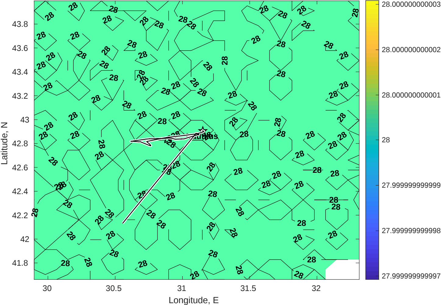
Surface Salinity for Nautilus at 08-Jan-2026 00:00:00
