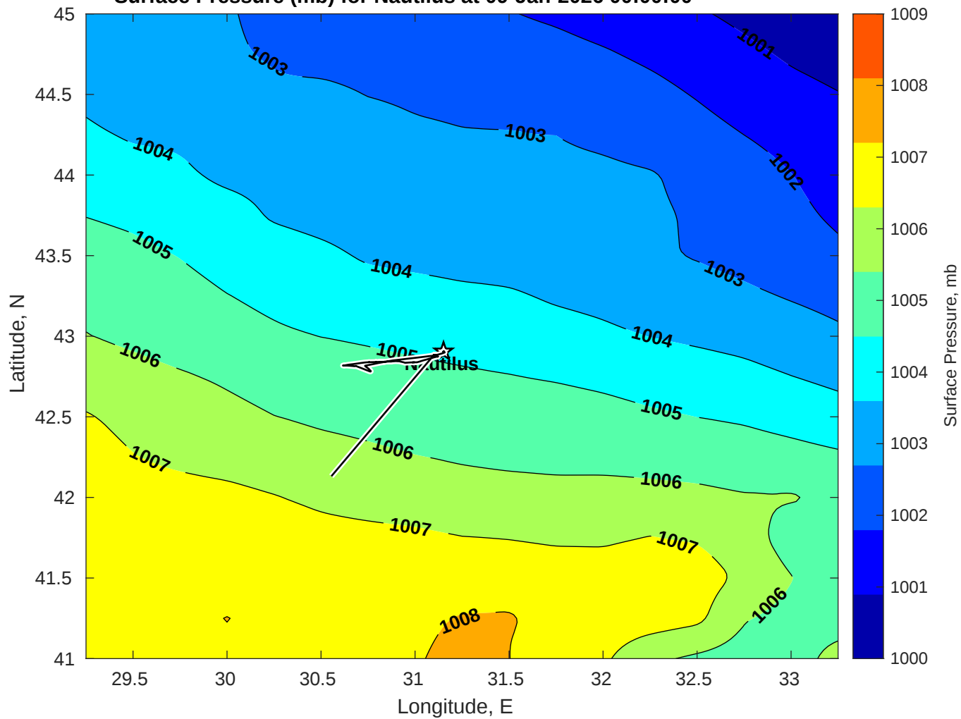
Surface Pressure (mb) for Nautilus at 09-Jan-2026 00:00:00
