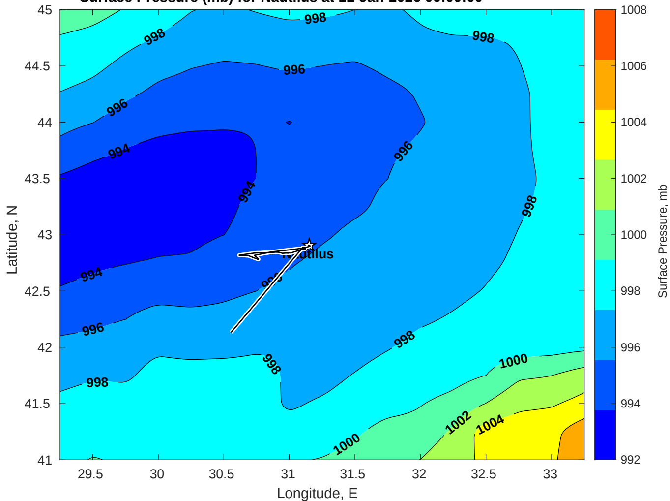
Surface Pressure (mb) for Nautilus at 11-Jan-2026 00:00:00
