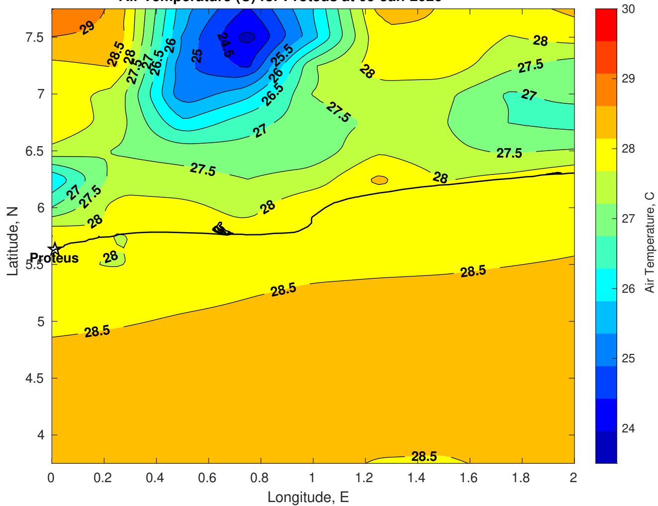
Air Temperature (C) for Proteus at 09-Jan-2026
