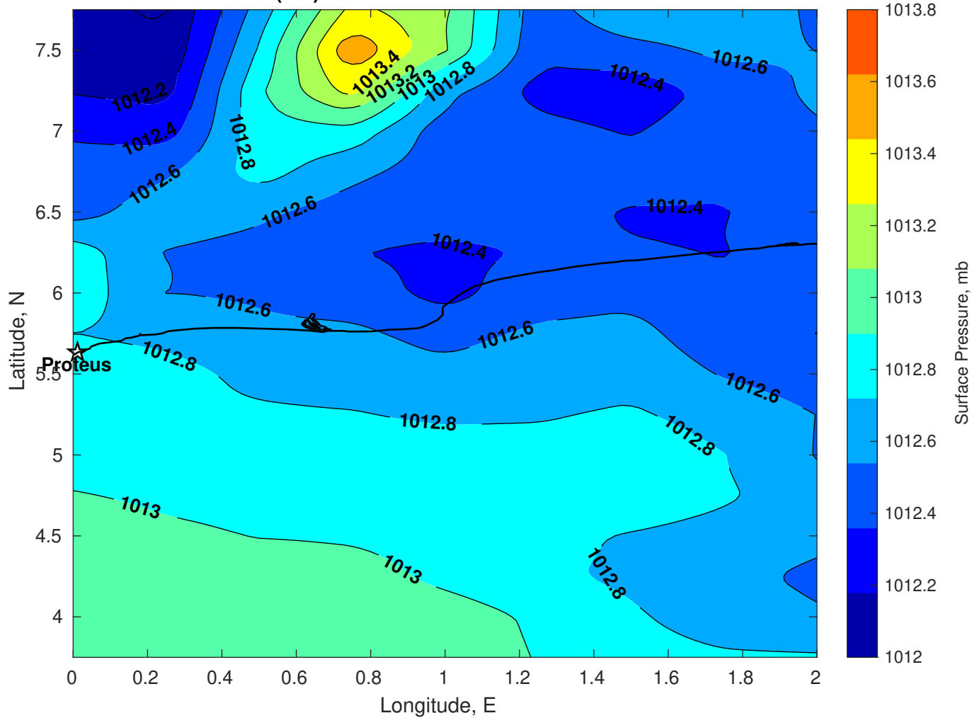
Surface Pressure (mb) for Proteus at 09-Jan-2026 00:00:00
