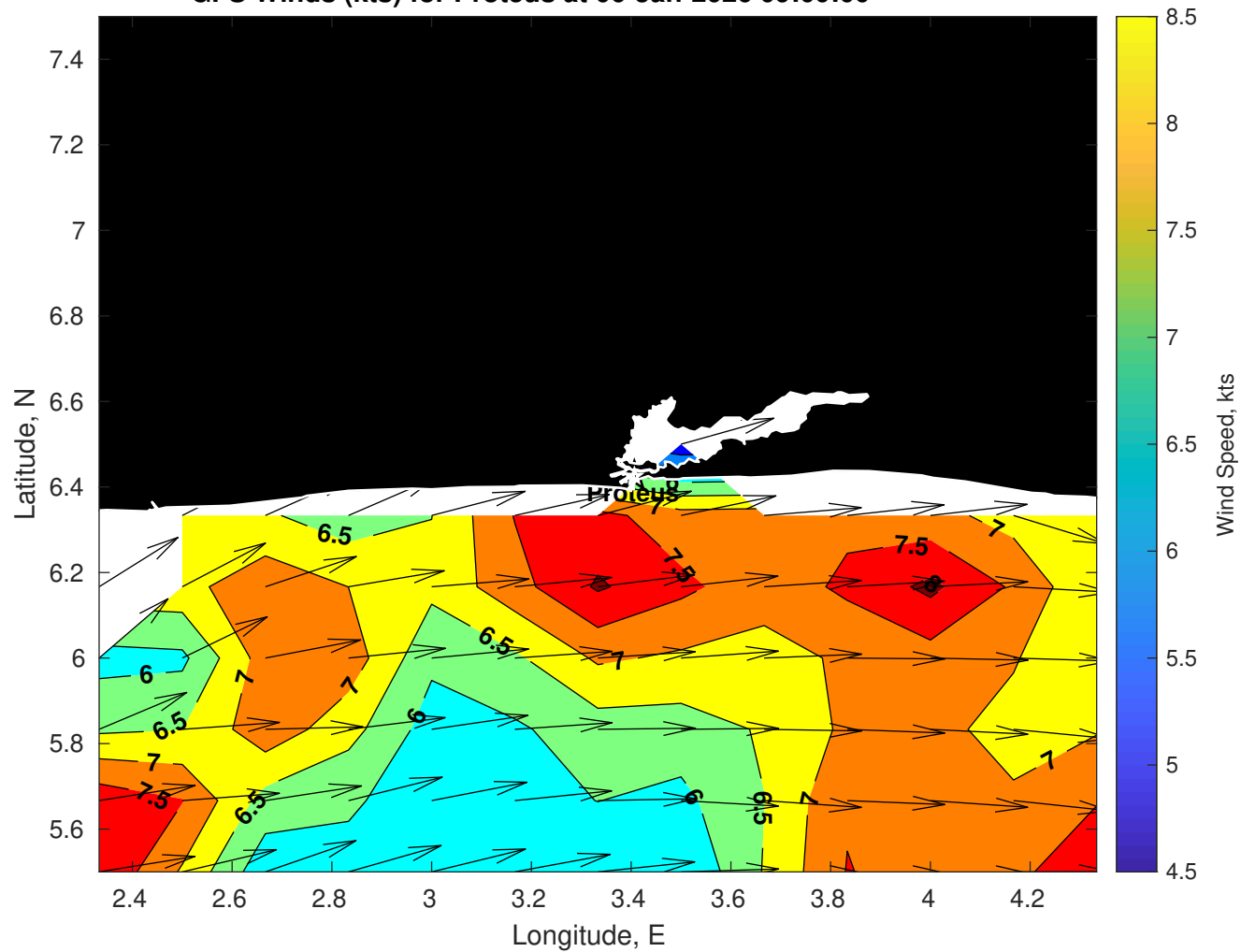
GFS Winds (kts) for Proteus at 06-Jan-2026 09:00:00
