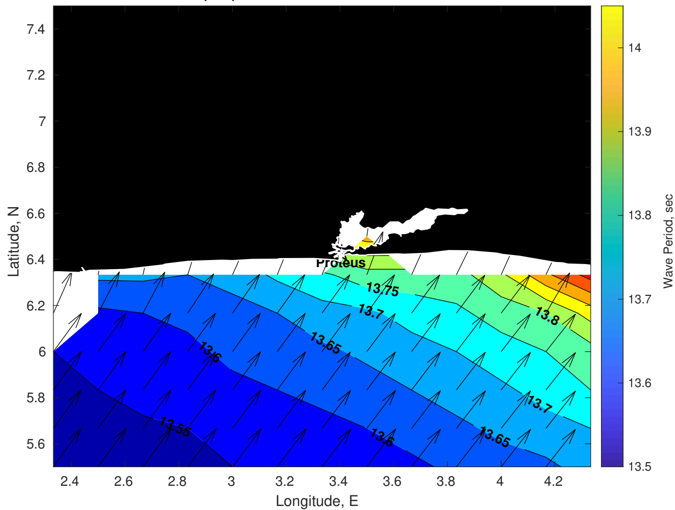
GFS Wave Period (sec) for Proteus at 06-Jan-2026 09:00:00
