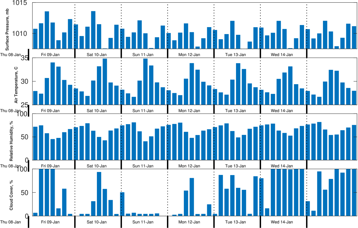
Met Forecast for Proteus from 09-Jan-2026 00:00:00 to 16-Jan-2026 00:00:00
