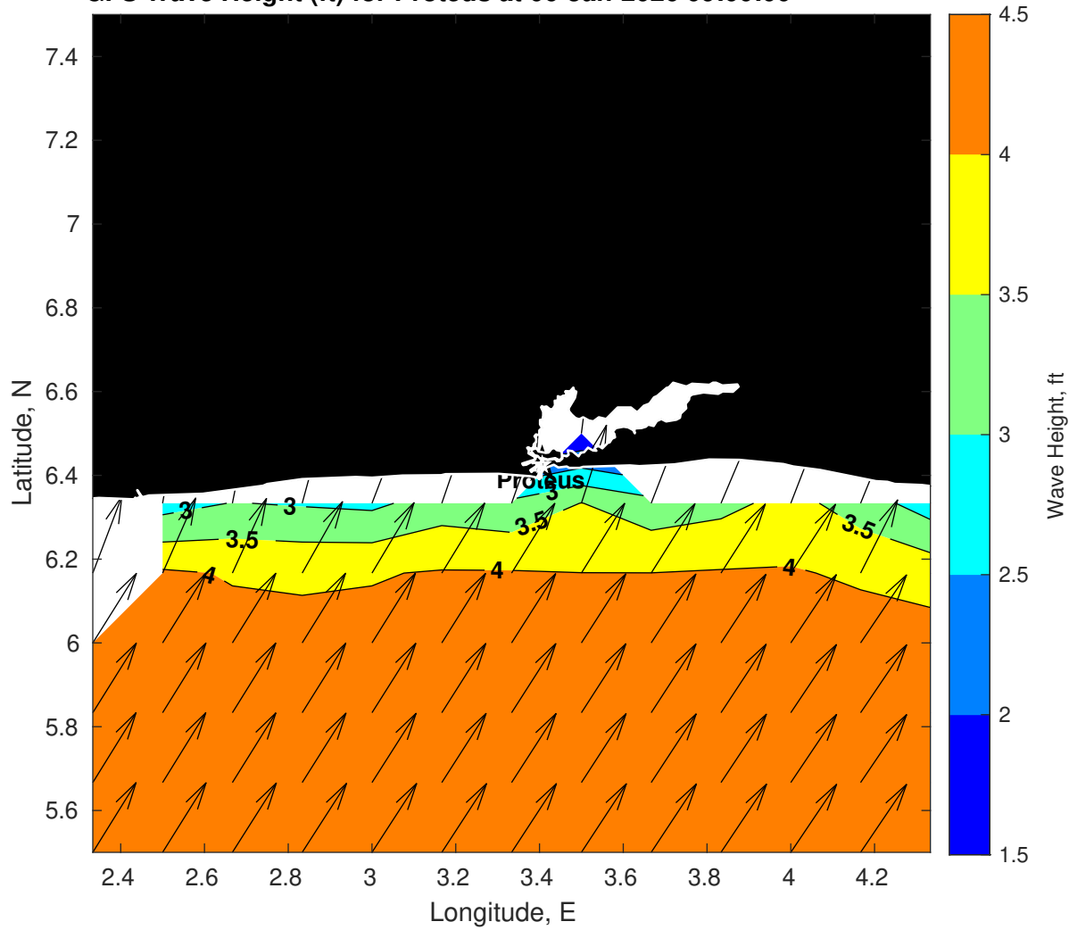
GFS Wave Height (ft) for Proteus at 06-Jan-2026 09:00:00
