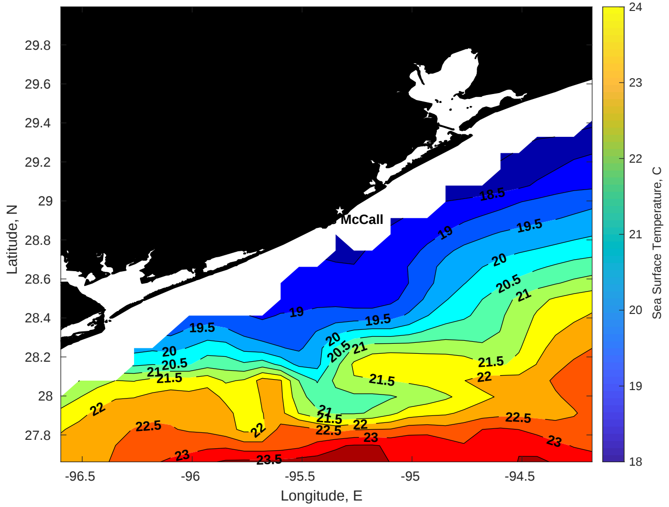
SST for Brooks McCall at 09-Jan-2026 00:00:00
