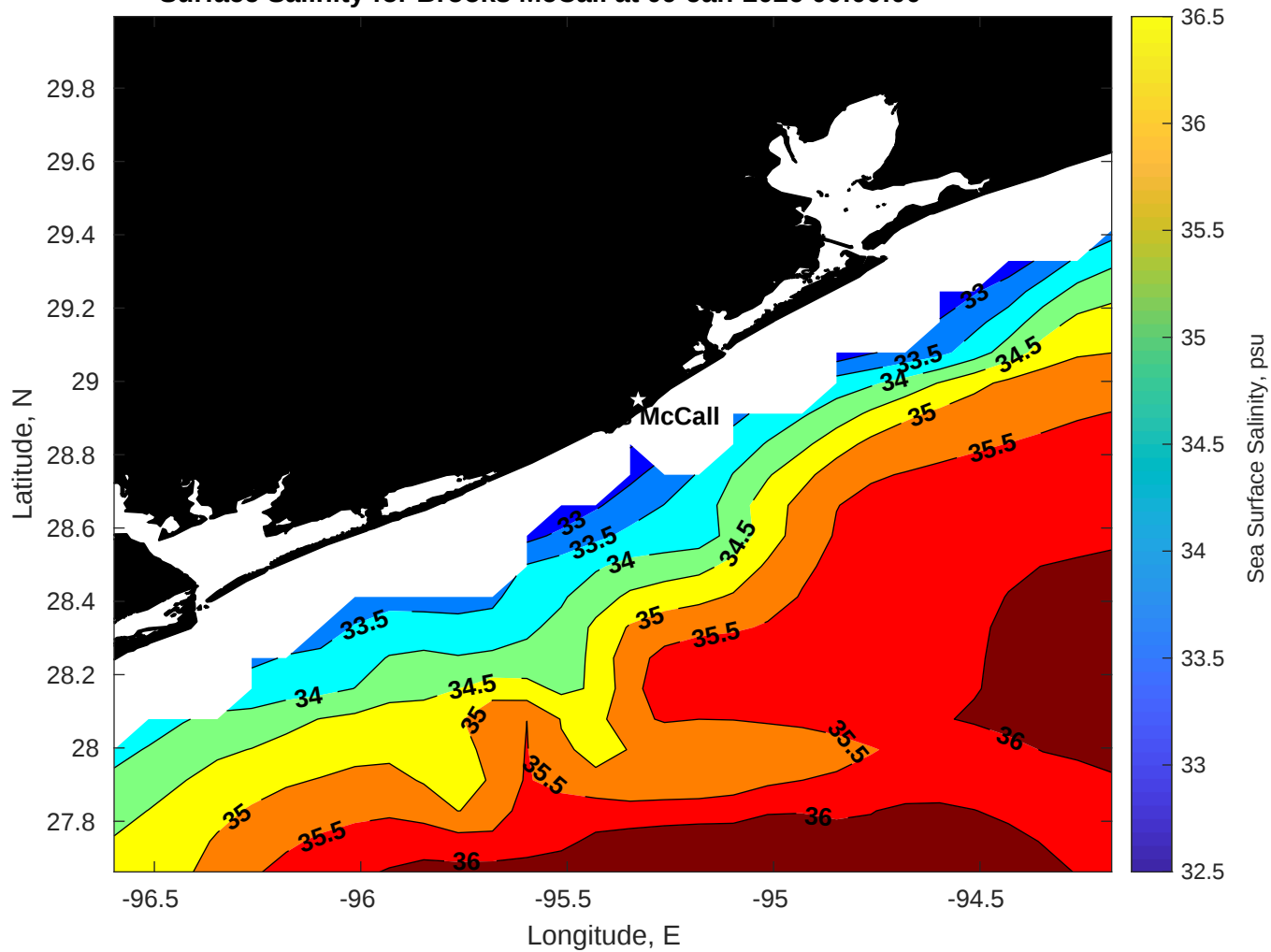
Surface Salinity for Brooks McCall at 09-Jan-2026 00:00:00
