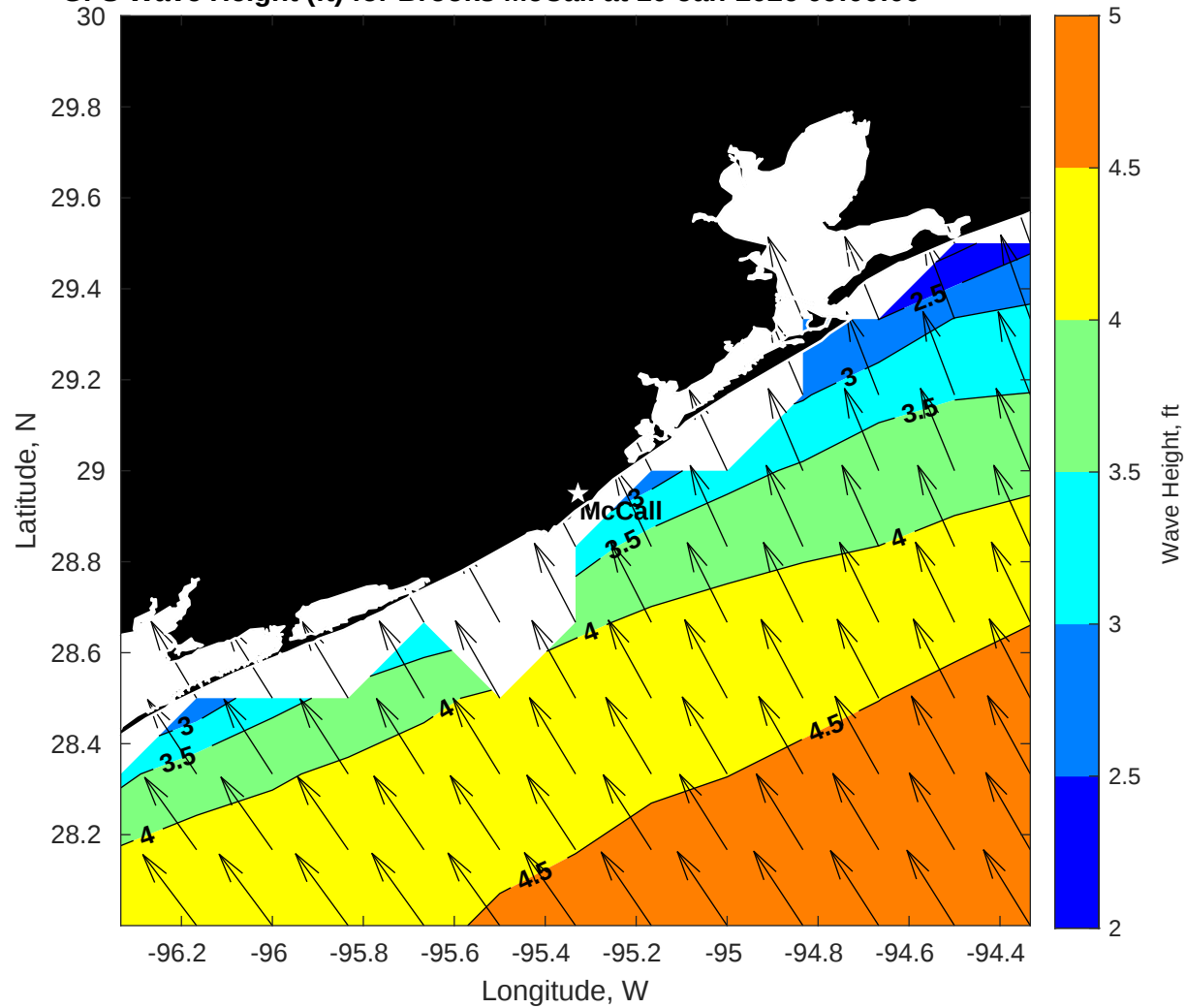
GFS Wave Height (ft) for Brooks McCall at 10-Jan-2026 09:00:00
