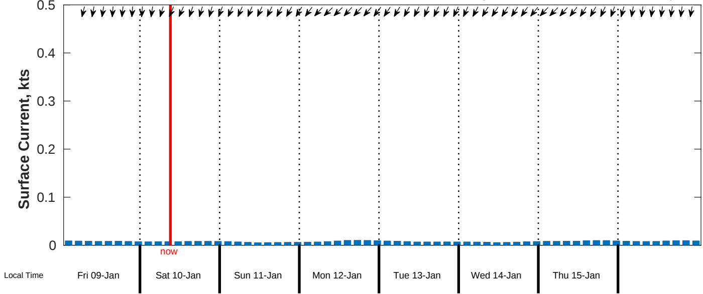
Surface Current Forecast for CSA (ONHYM) PPL EBS - Ghana from 09-Jan-2026 00:00:00 to 17-Jan-2026 00:00:00
