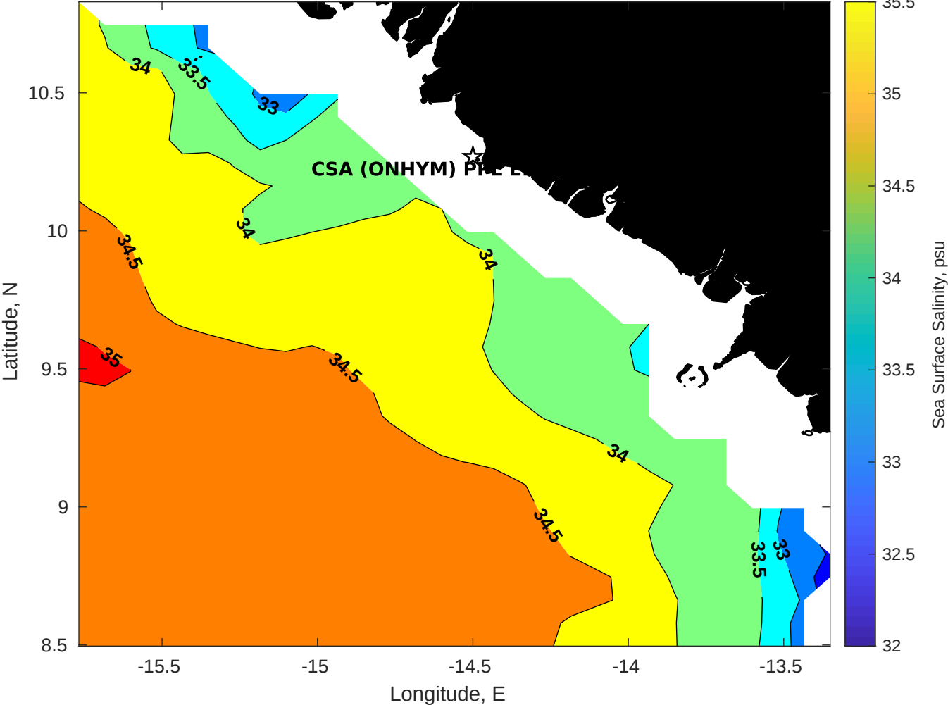
Surface Salinity for CSA (ONHYM) PPL EBS - Guinea at 09-Jan-2026 00:00:00
