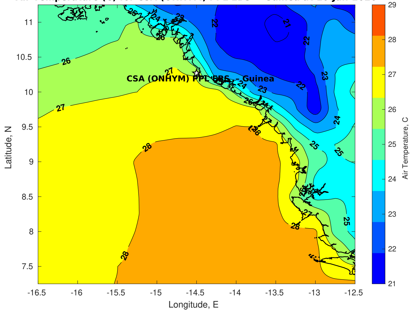
Air Temperature (C) for CSA (ONHYM) PPL EBS - Guinea at 10-Jan-2026
