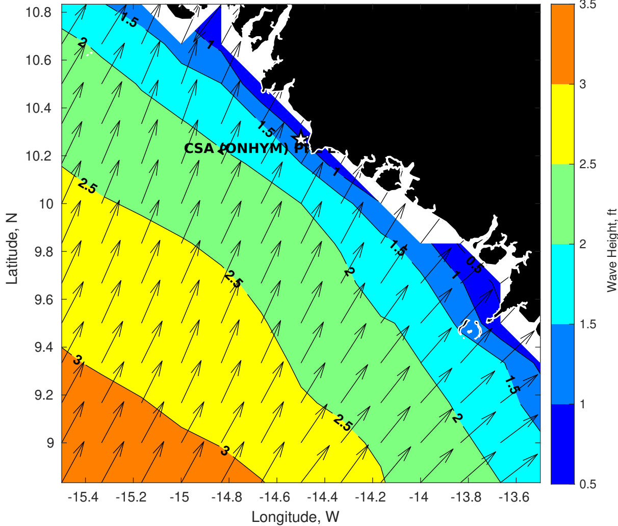
GFS Wave Height (ft) for CSA (ONHYM) PPL EBS - Guinea at 10-Jan-2026 09:00:00
