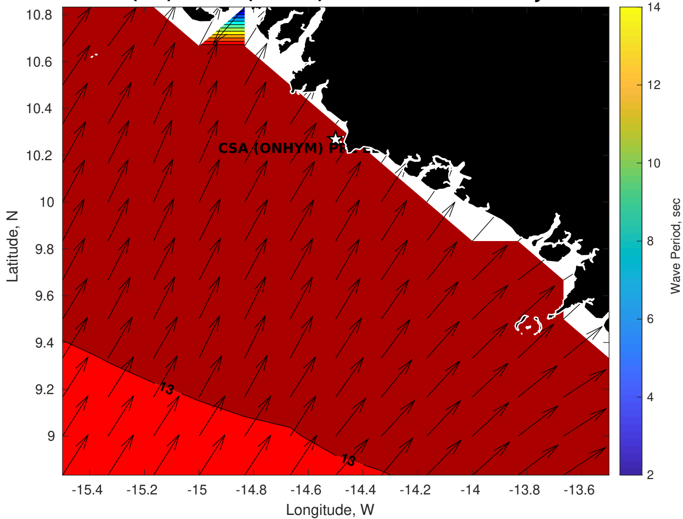
GFS Wave Period (sec) for CSA (ONHYM) PPL EBS - Guinea at 10-Jan-2026 09:00:00
