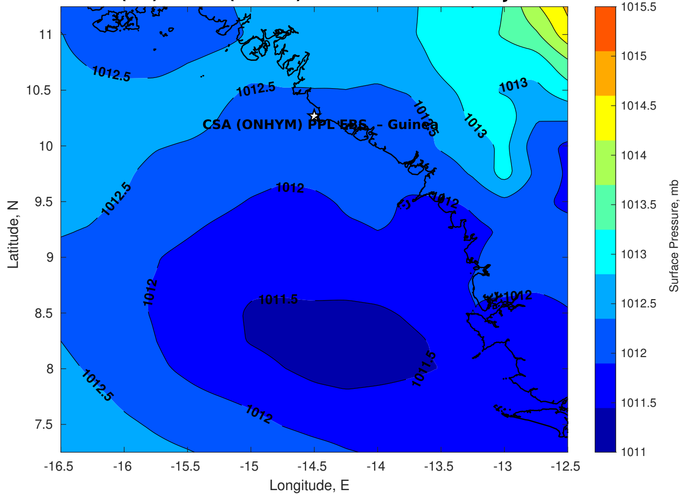
Surface Pressure (mb) for CSA (ONHYM) PPL EBS - Guinea at 11-Jan-2026 00:00:00
