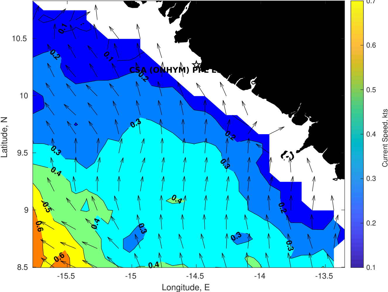
Surface Currents for CSA (ONHYM) PPL EBS - Guinea at 09-Jan-2026 00:00:00
