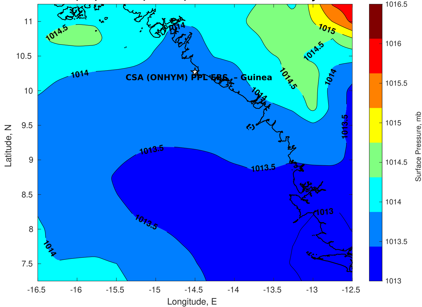
Surface Pressure (mb) for CSA (ONHYM) PPL EBS - Guinea at 10-Jan-2026 00:00:00
