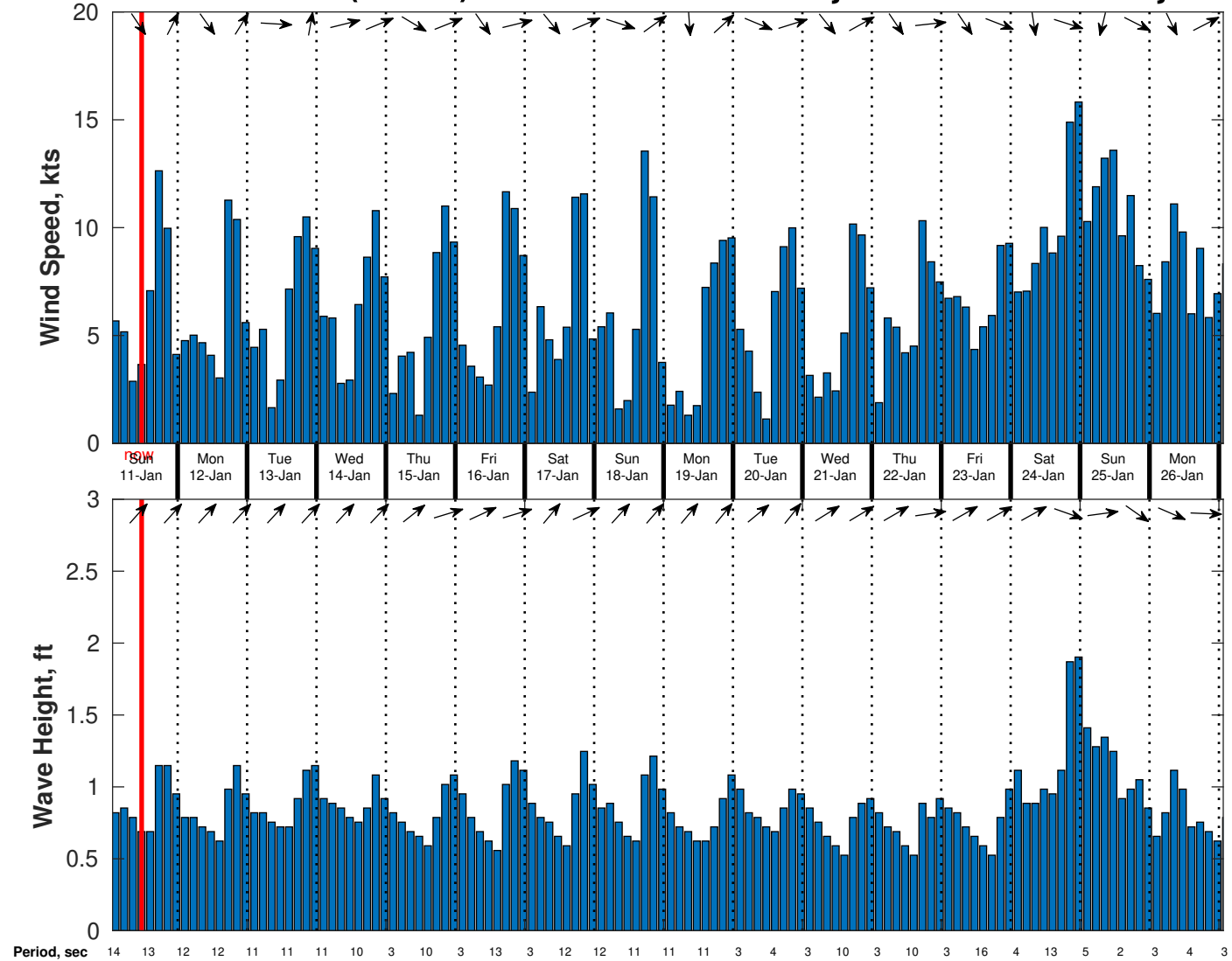
Wind & Wave Forecast for CSA (ONHYM) PPL EBS - Guinea from 10-Jan-2026 01:00:00 to 26-Jan-2026 01:00:00
