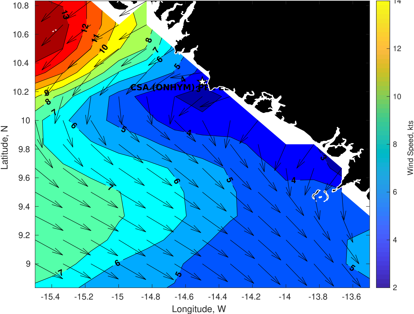
GFS Winds (kts) for CSA (ONHYM) PPL EBS - Guinea at 10-Jan-2026 09:00:00
