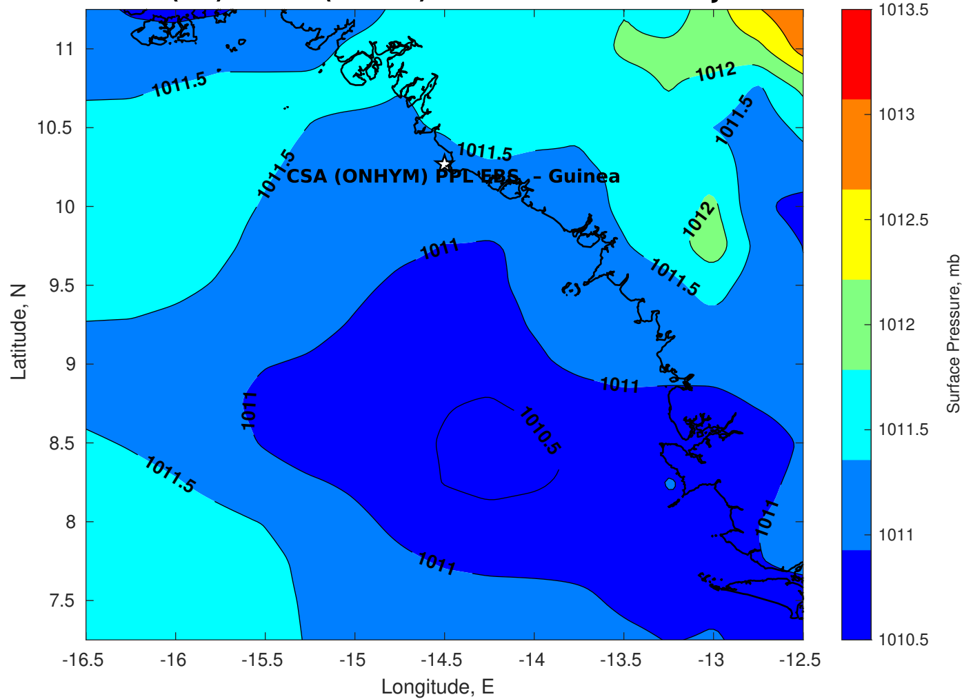
Surface Pressure (mb) for CSA (ONHYM) PPL EBS - Guinea at 12-Jan-2026 00:00:00
