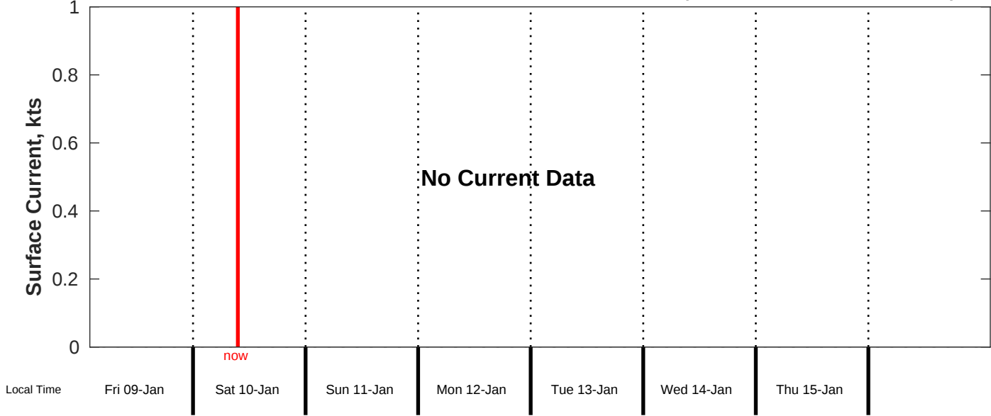
Surface Current Forecast for CSA (ONHYM) PPL EBS - Guinea from 09-Jan-2026 00:00:00 to 17-Jan-2026 00:00:00
