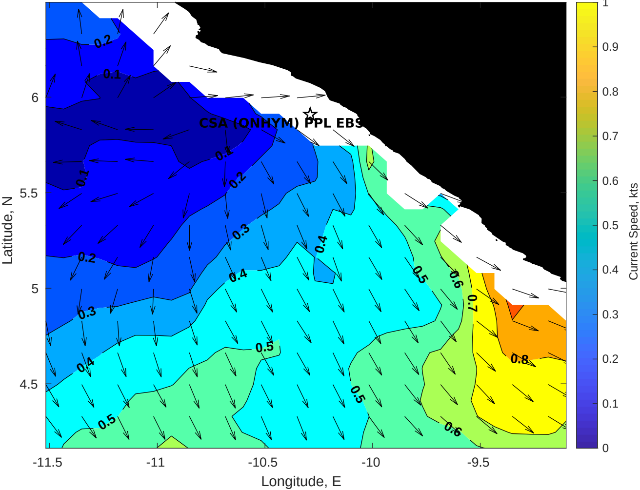
Surface Currents for CSA (ONHYM) PPL EBS - Liberia at 09-Jan-2026 00:00:00
