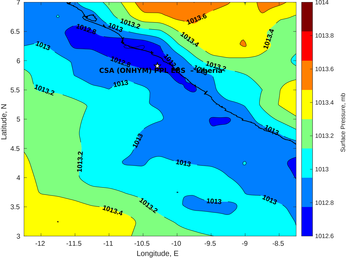
Surface Pressure (mb) for CSA (ONHYM) PPL EBS - Liberia at 10-Jan-2026 00:00:00
