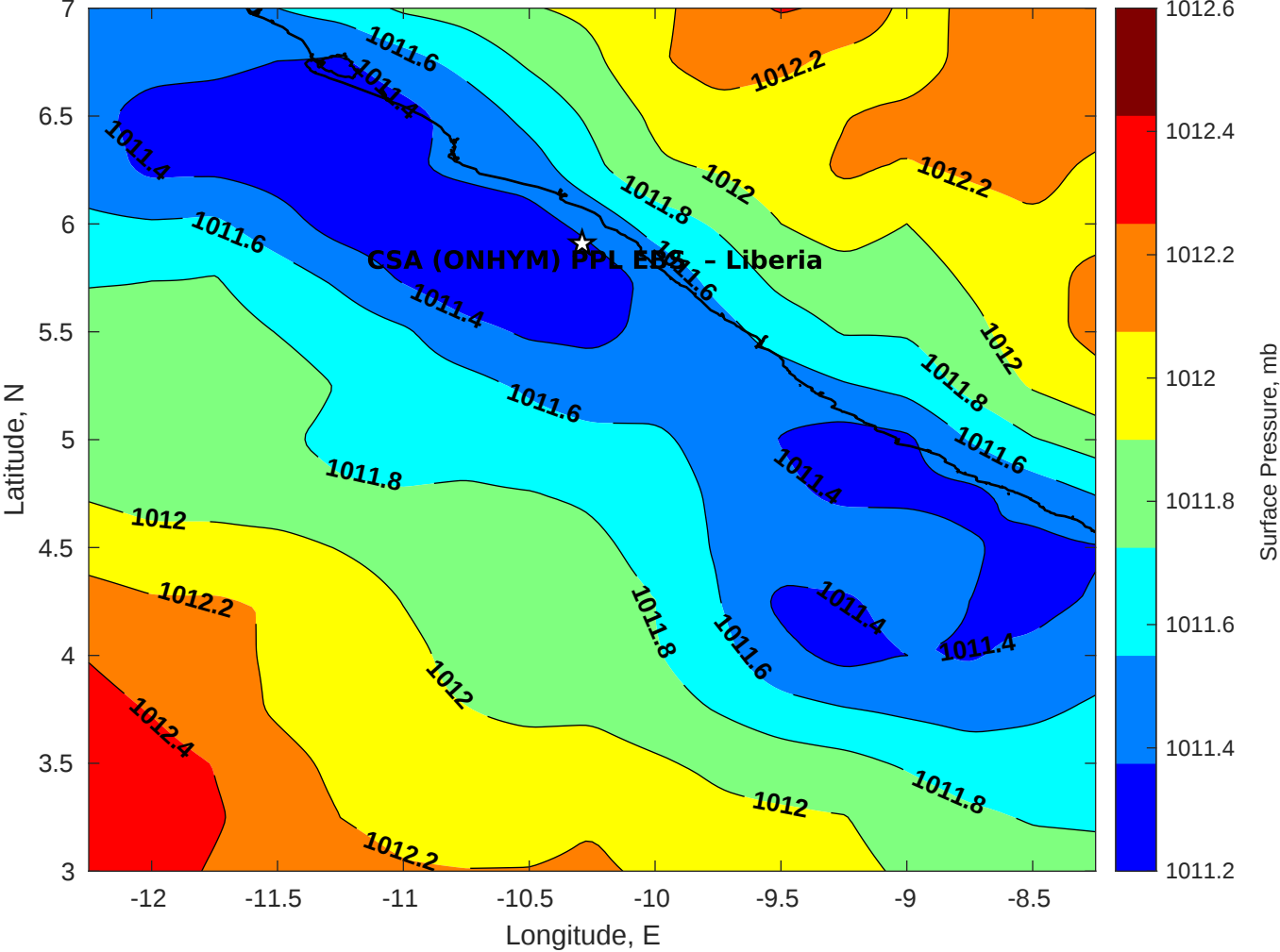
Surface Pressure (mb) for CSA (ONHYM) PPL EBS - Liberia at 11-Jan-2026 00:00:00
