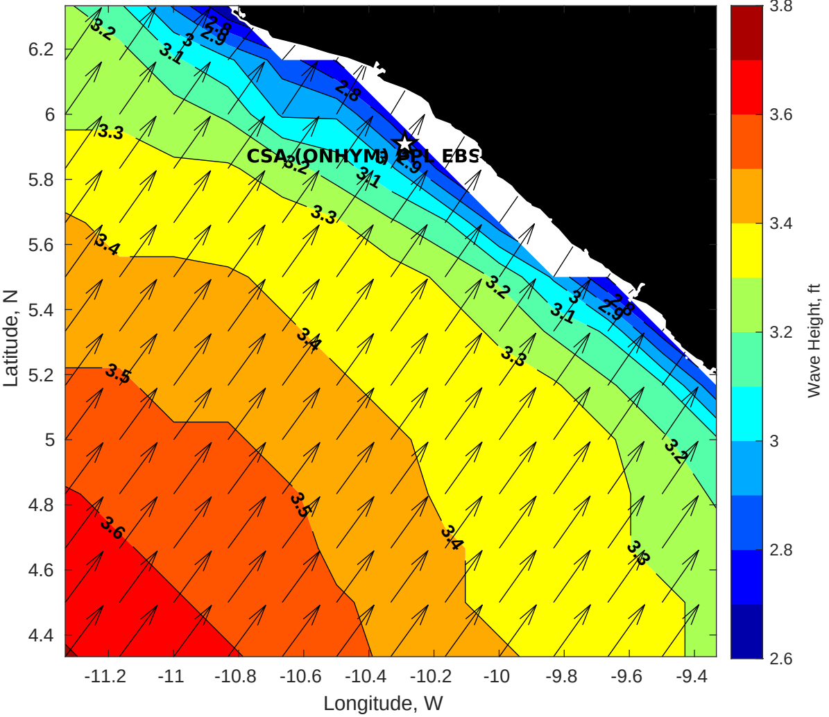
GFS Wave Height (ft) for CSA (ONHYM) PPL EBS - Liberia at 10-Jan-2026 09:00:00
