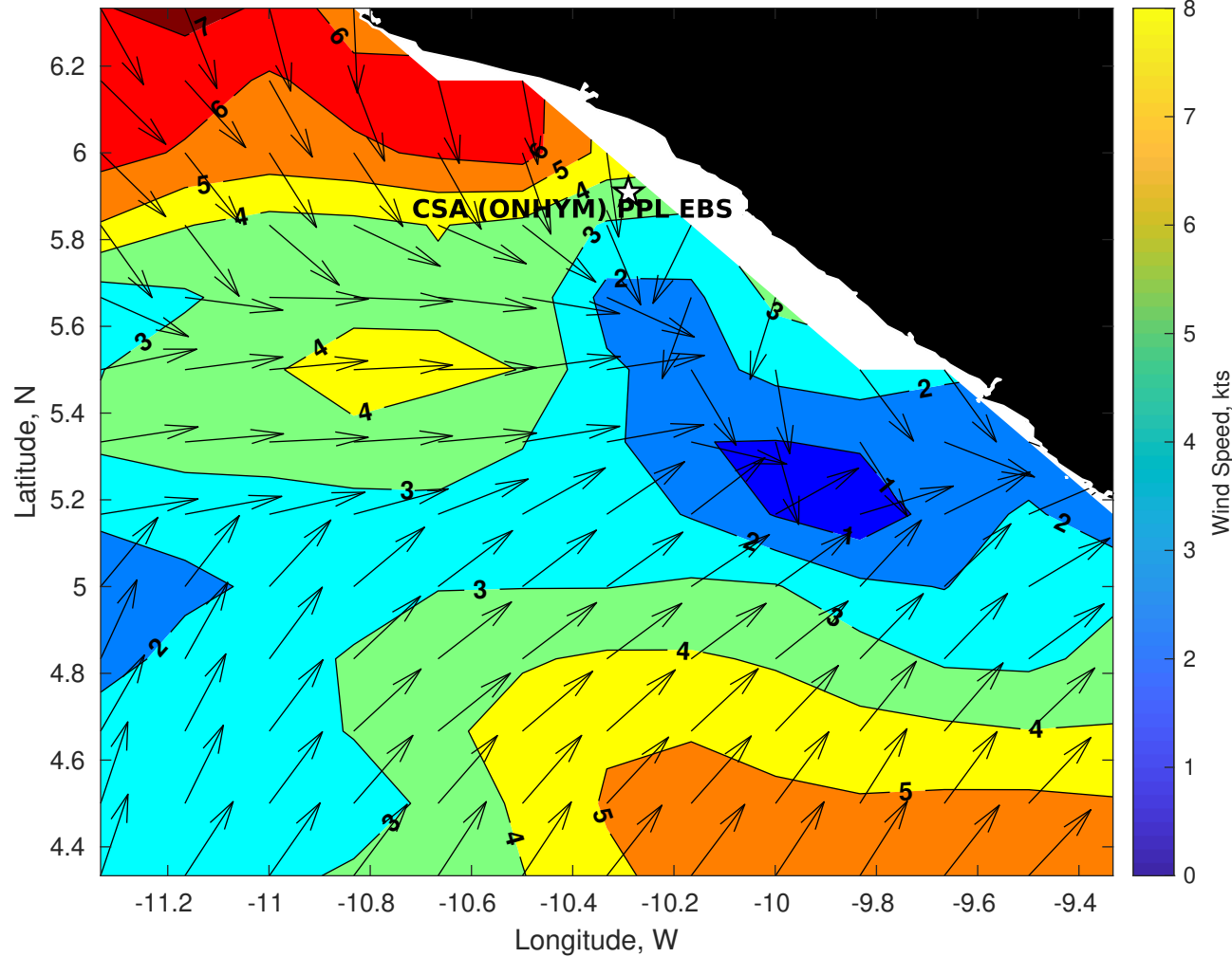
GFS Winds (kts) for CSA (ONHYM) PPL EBS - Liberia at 10-Jan-2026 09:00:00
