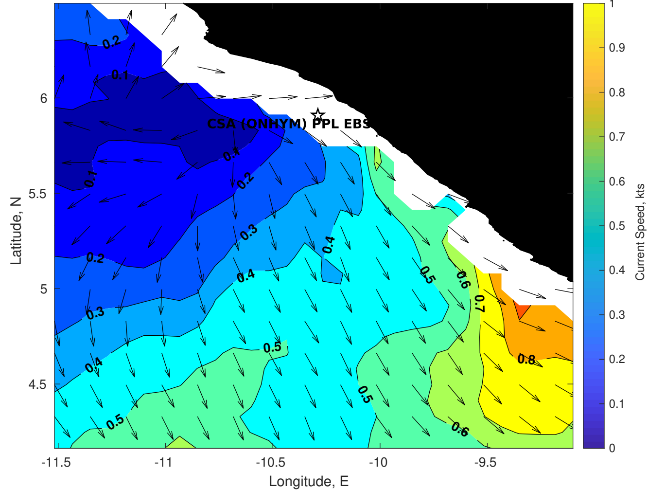
Surface Currents for CSA (ONHYM) PPL EBS - Liberia at 09-Jan-2026 00:00:00
