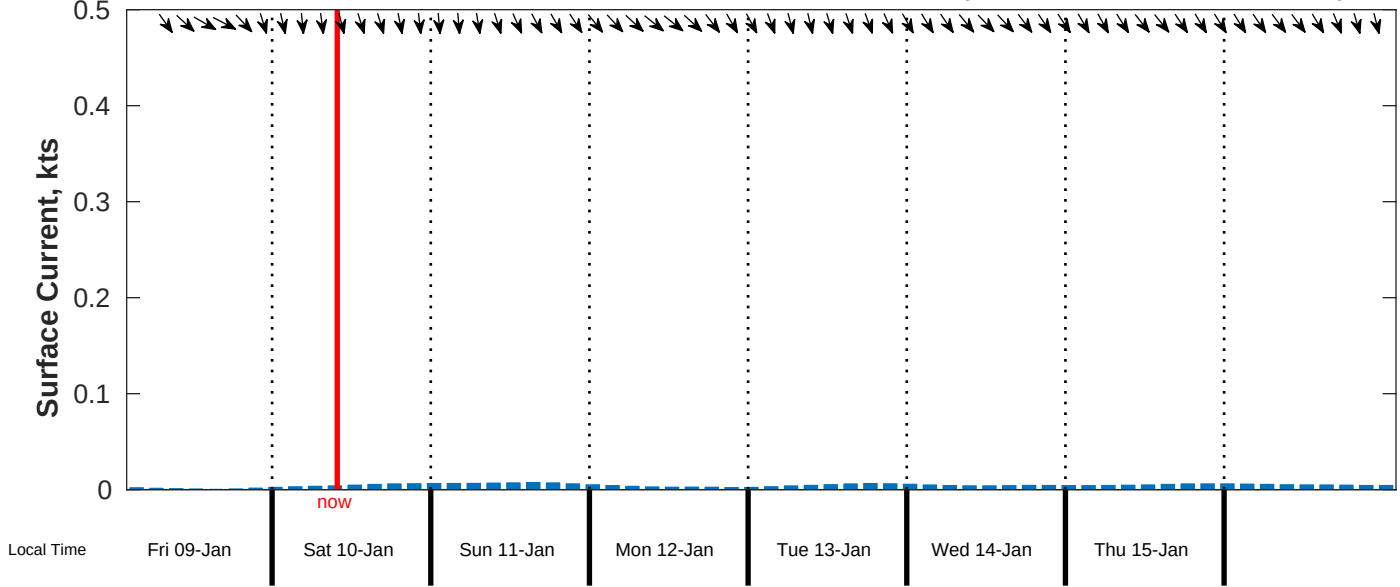
Surface Current Forecast for CSA (ONHYM) PPL EBS - Liberia from 09-Jan-2026 00:00:00 to 17-Jan-2026 00:00:00
