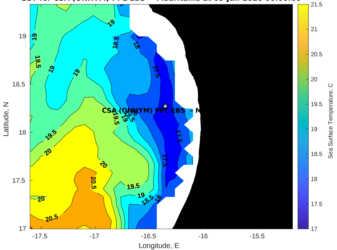
SST for CSA (ONHYM) PPL EBS - Mauritania at 09-Jan-2026 00:00:00
