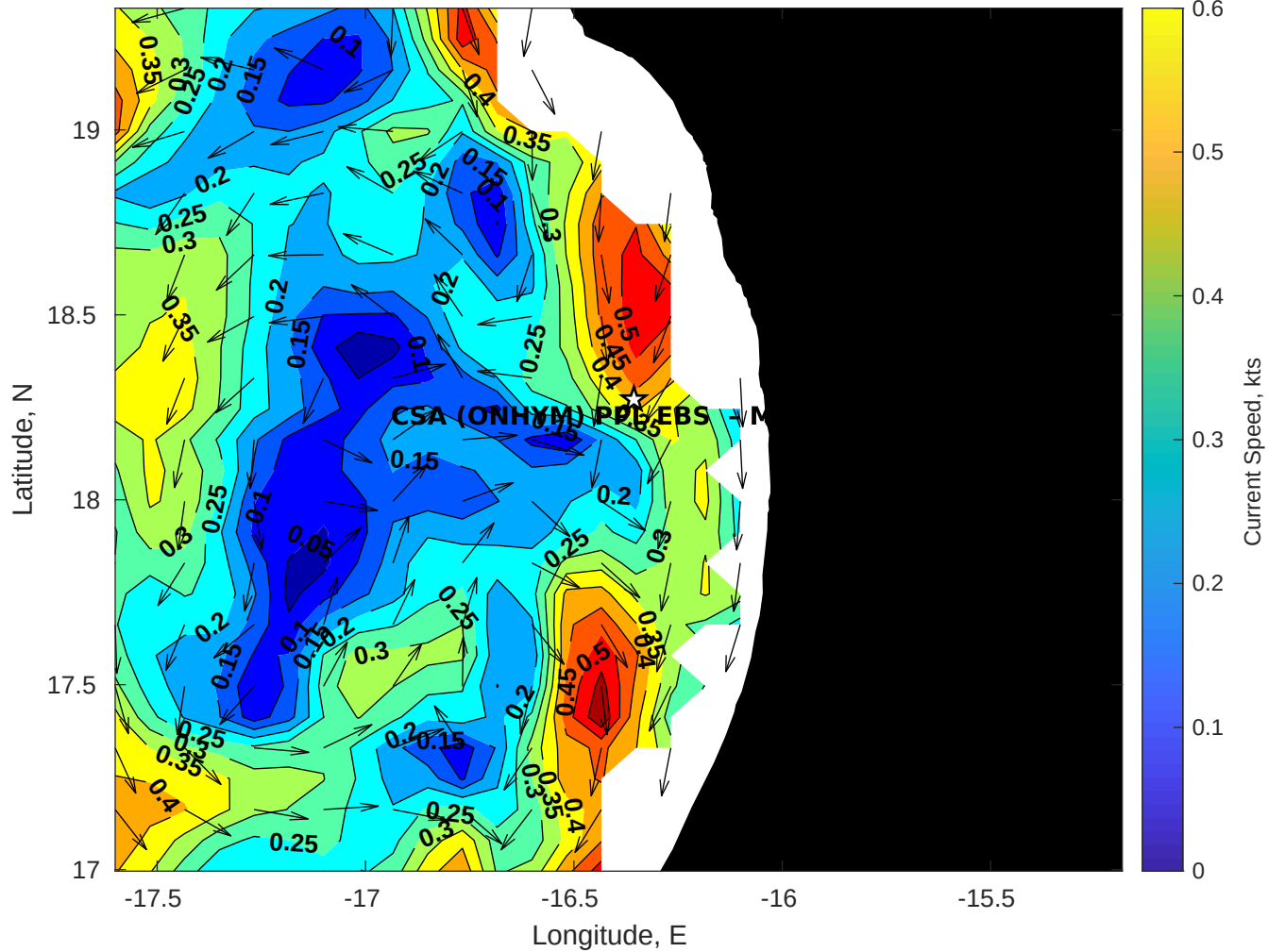
Surface Currents for CSA (ONHYM) PPL EBS - Mauritania at 09-Jan-2026 00:00:00
