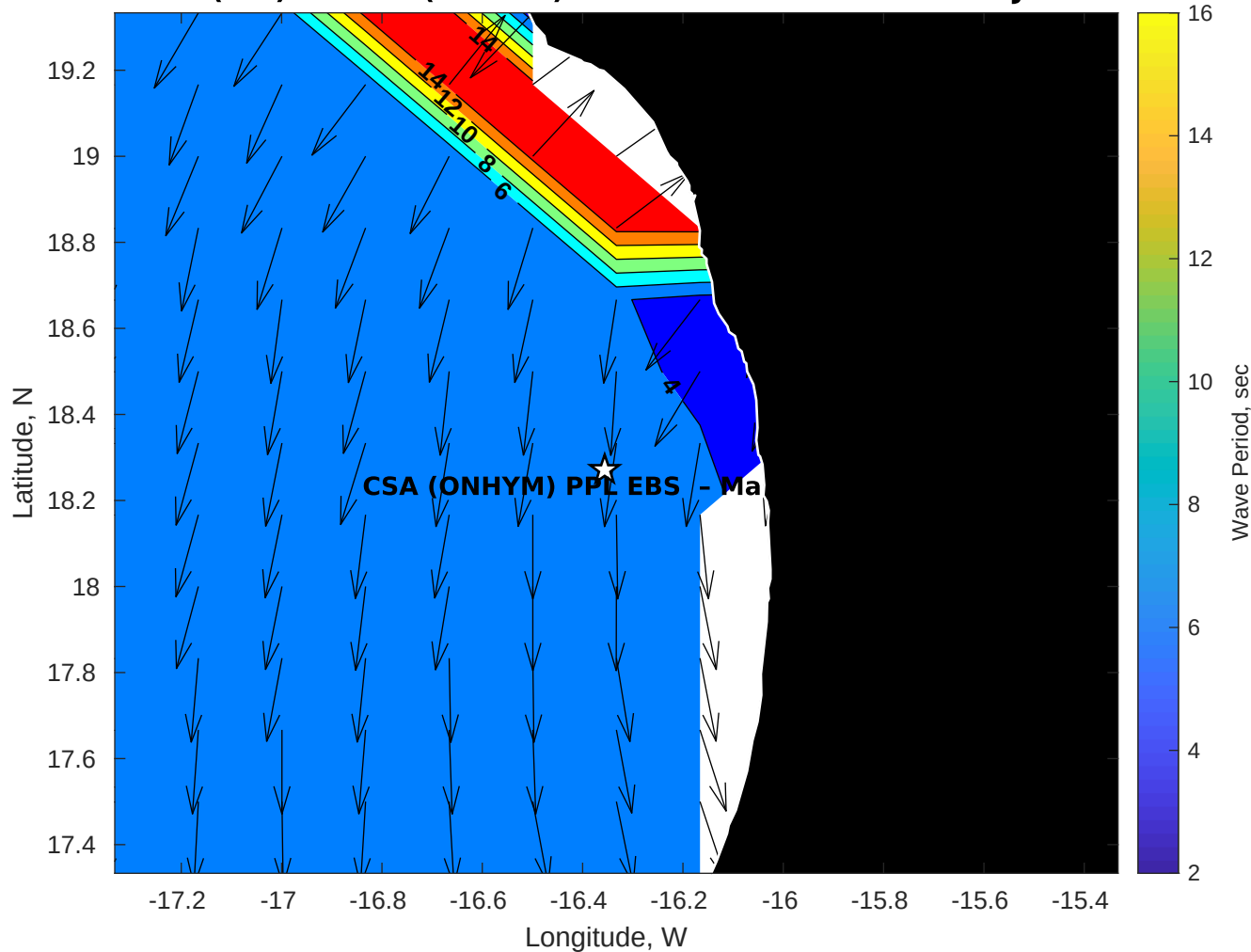
GFS Wave Period (sec) for CSA (ONHYM) PPL EBS - Mauritania at 10-Jan-2026 09:00:00
